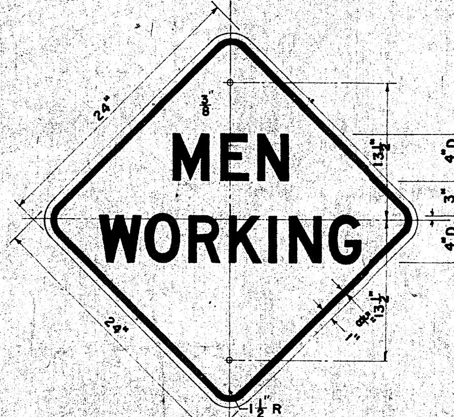
W-26 24"x24"
