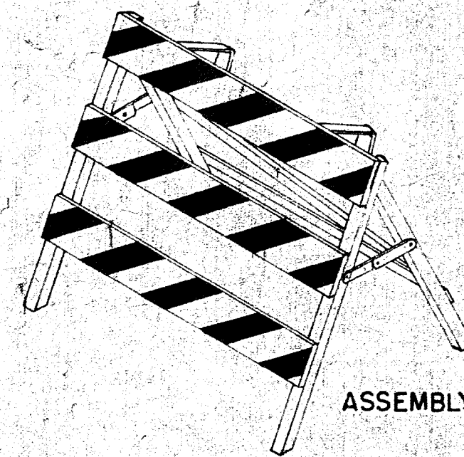
BARRICADE "G"
