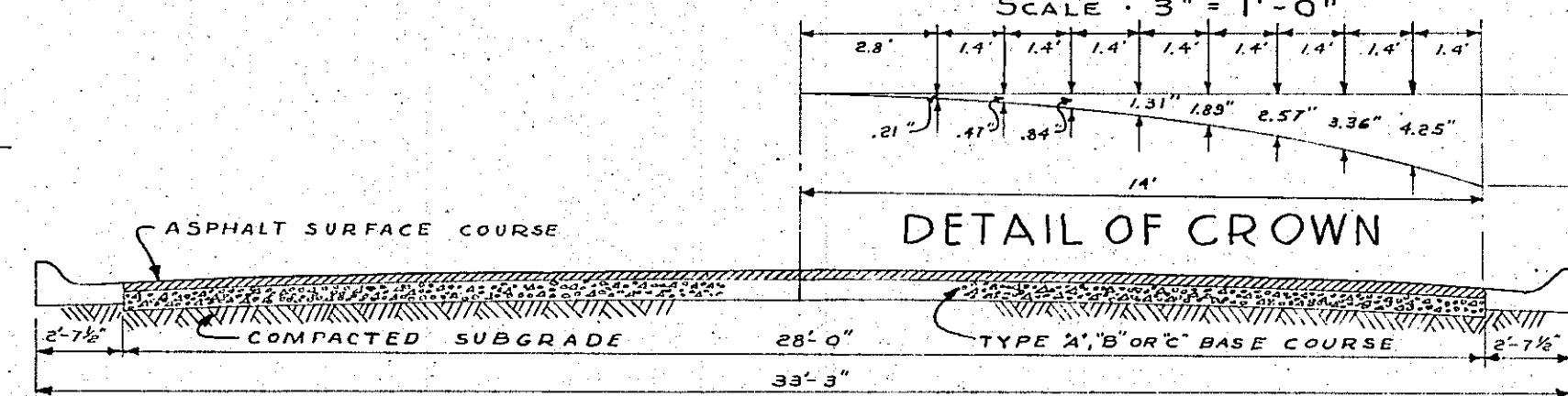
TYPICAL STREET SECTION NOT TO SCALE
