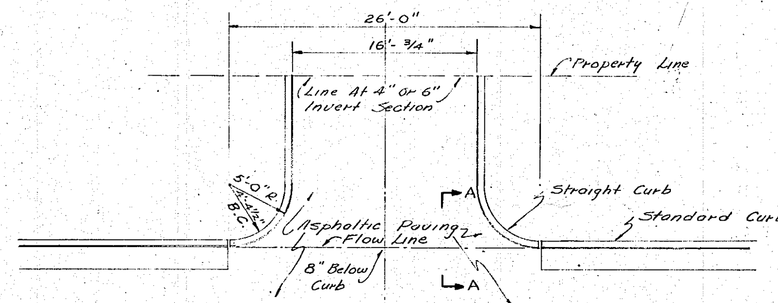
CURB RETURN TYPICAL STREET INTERSECTION SCALE: 1/8" = 1'-0"
