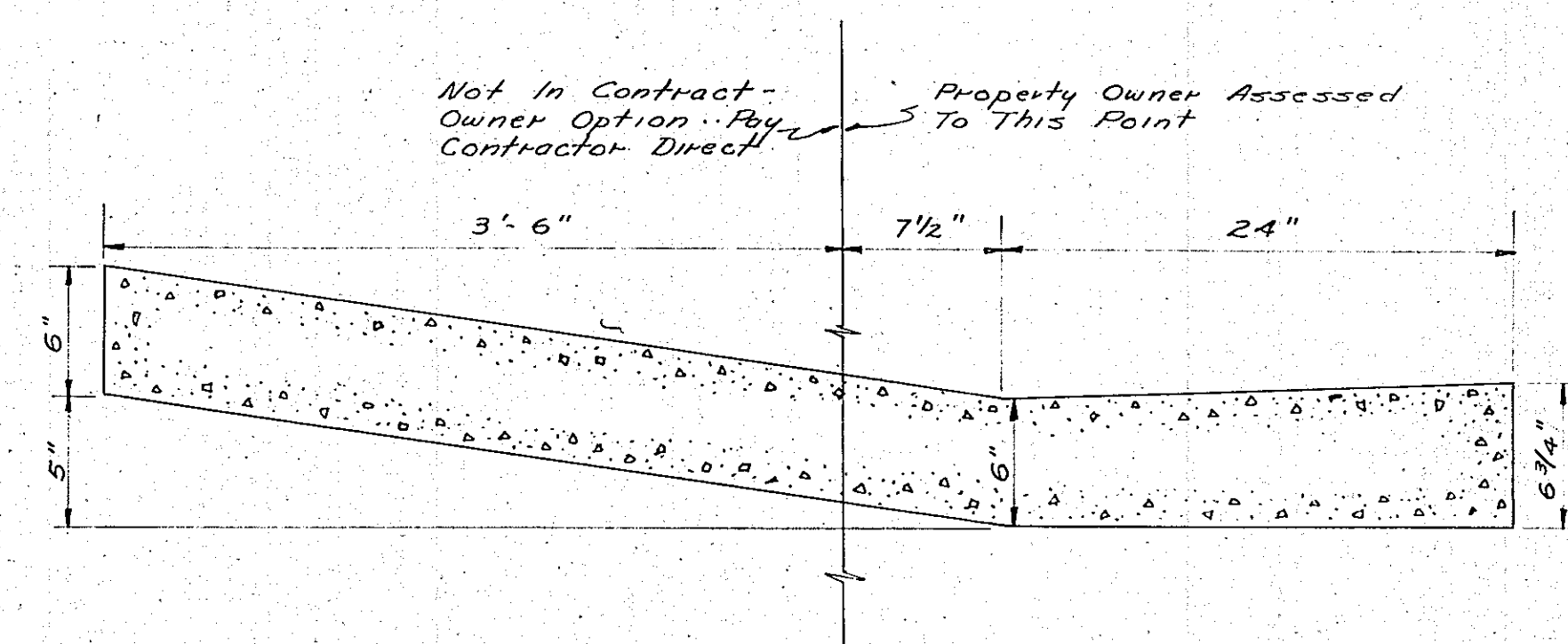
LAI D BACK GUTTER SCALE: 1/2" = 1'-0"
