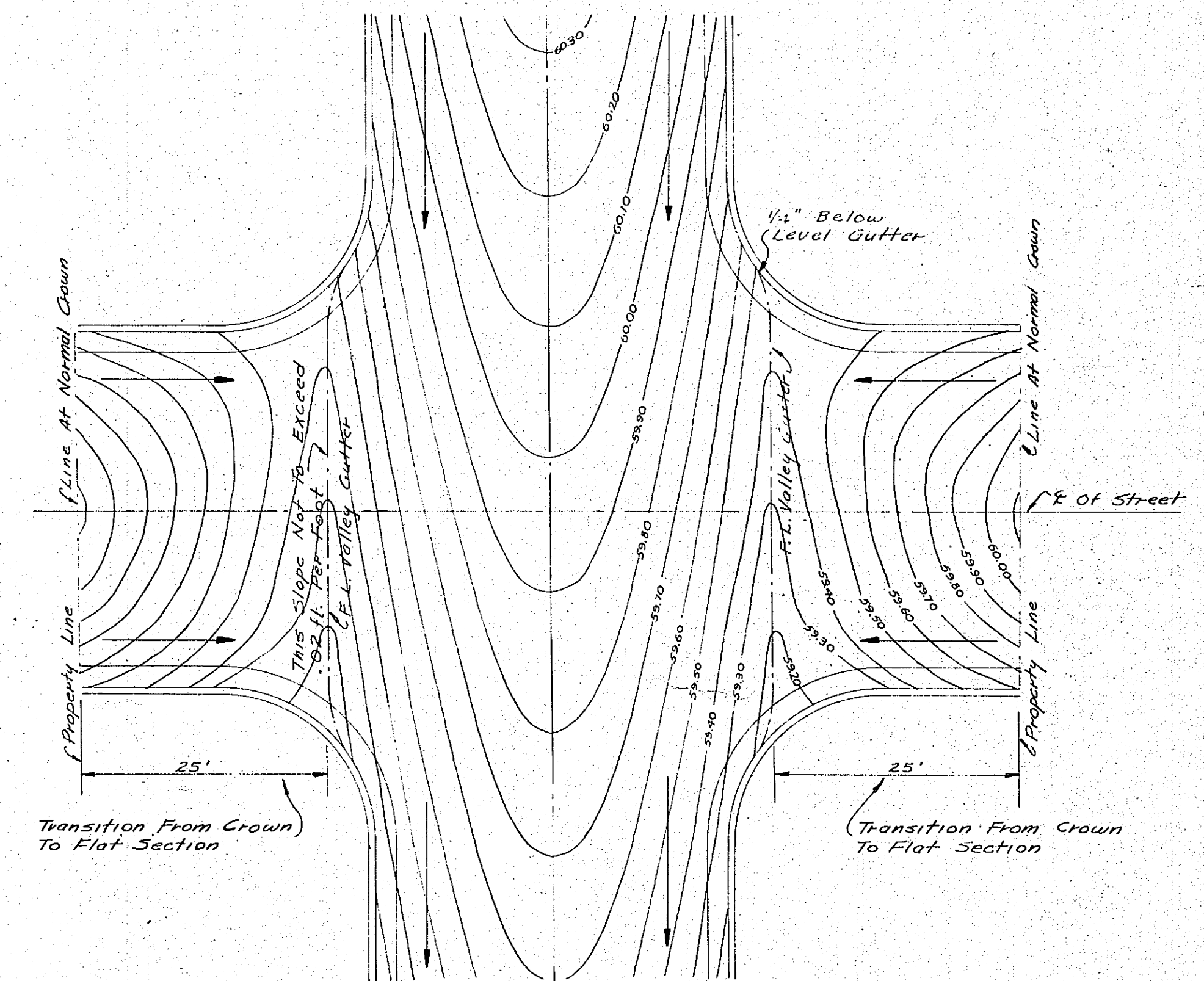
GRADE & VALLEY GUTTER TYPICAL STREET INTERSECTION SCALE: 3/32" = 1'-0"
