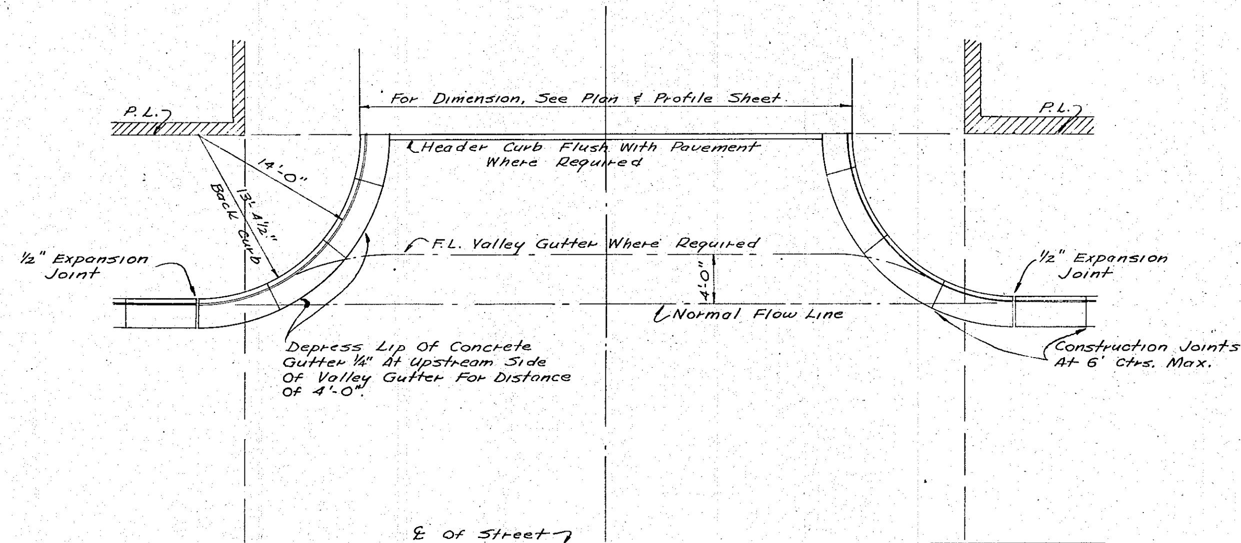
CURB RETURN TYPICAL STREET INTERSECTION SCALE: 1/8" = 1'-0"
