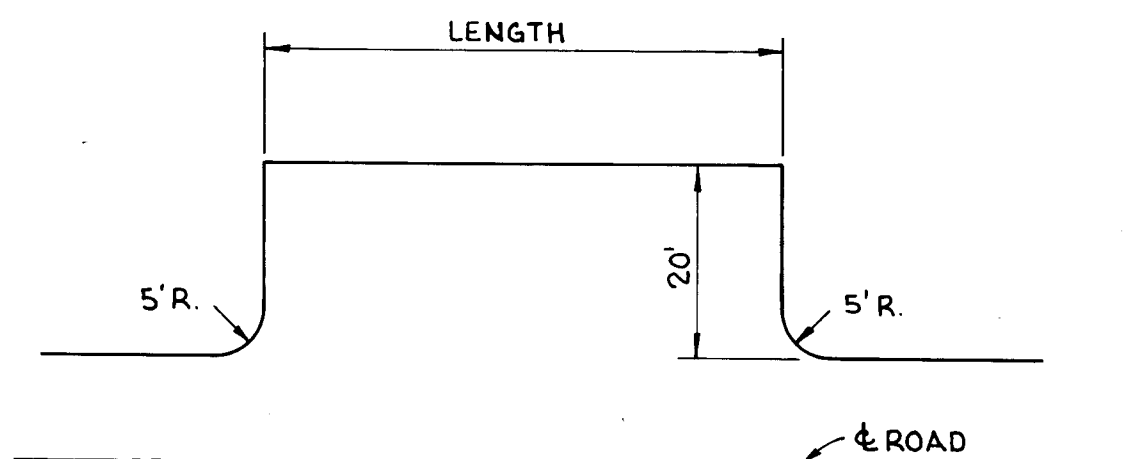
TYPICAL PARKING BAY See sheet 1A for length & location
