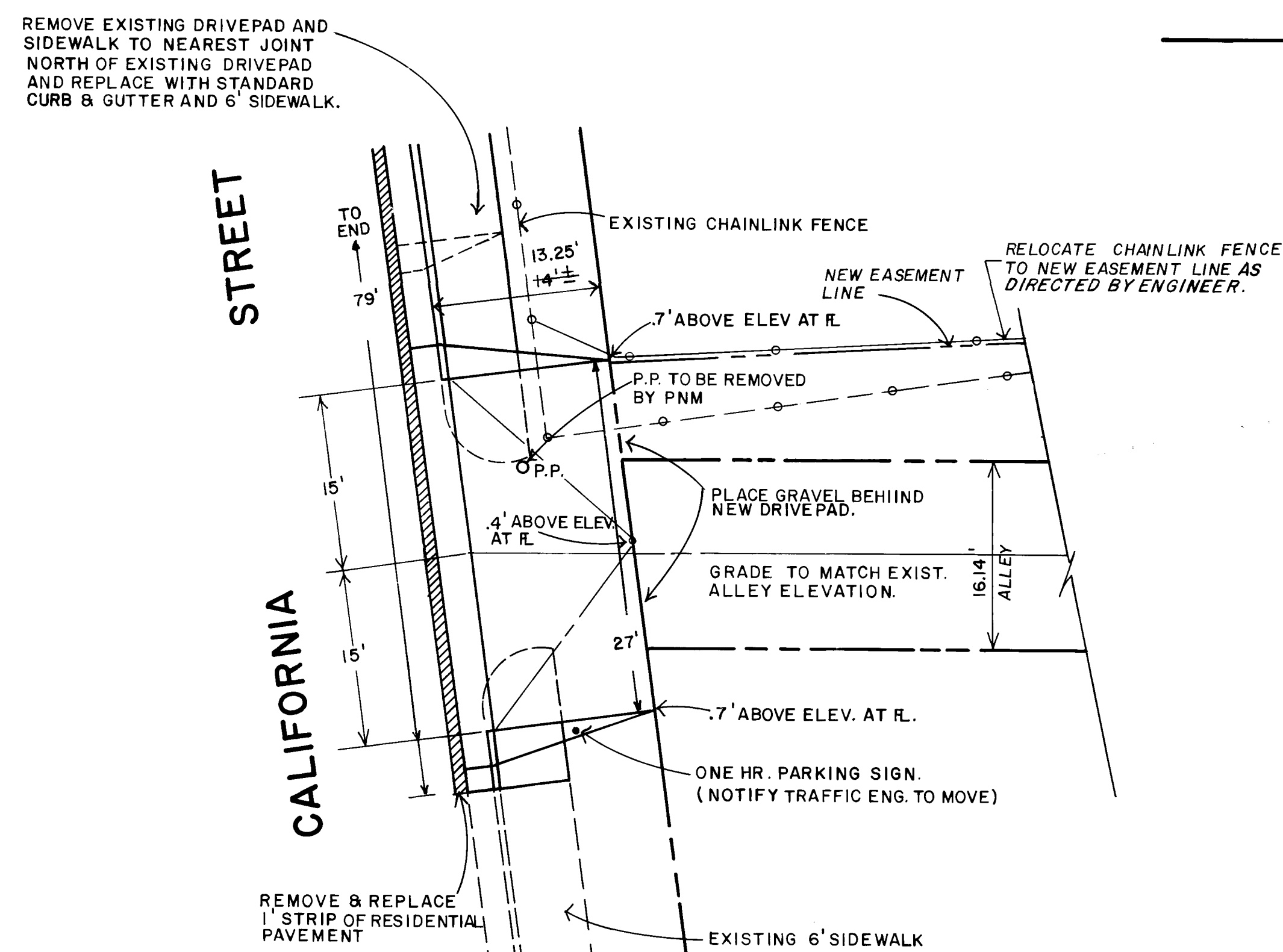
ALLEY DRIVEPAD DETAIL
