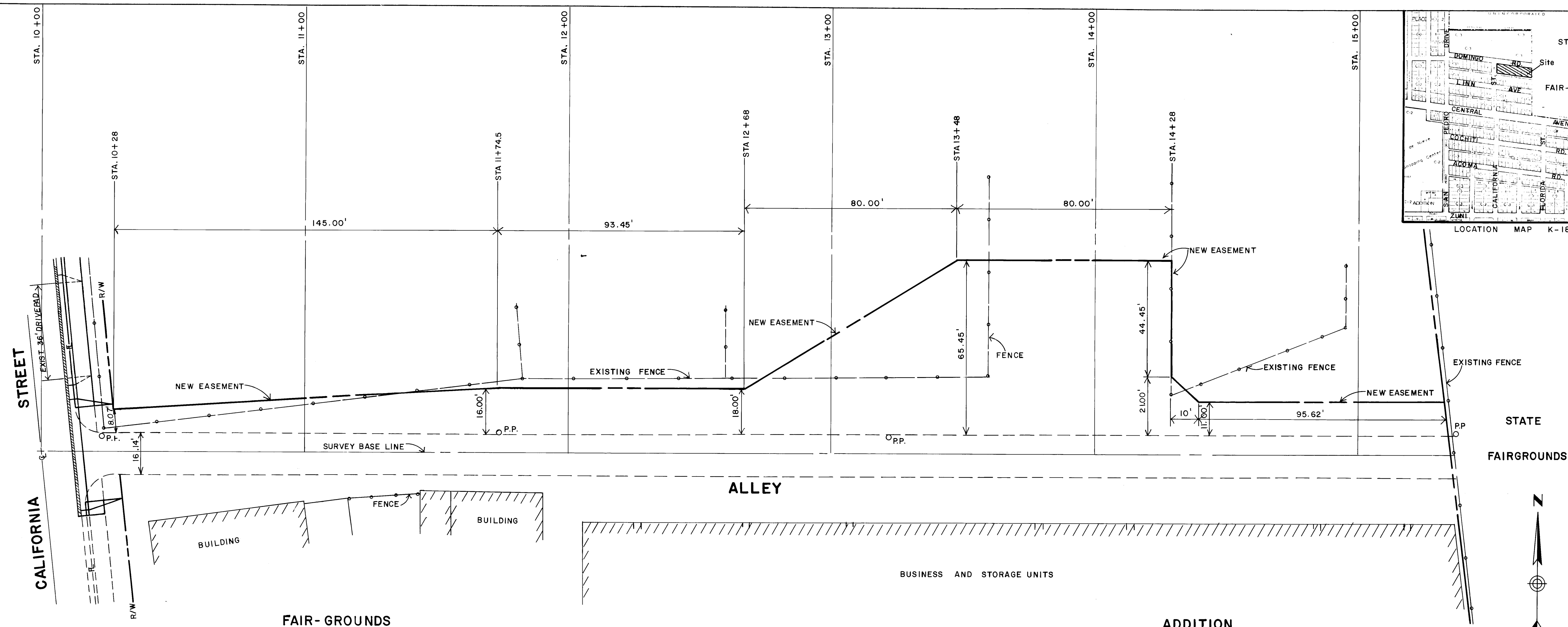
PLAN VIEW
