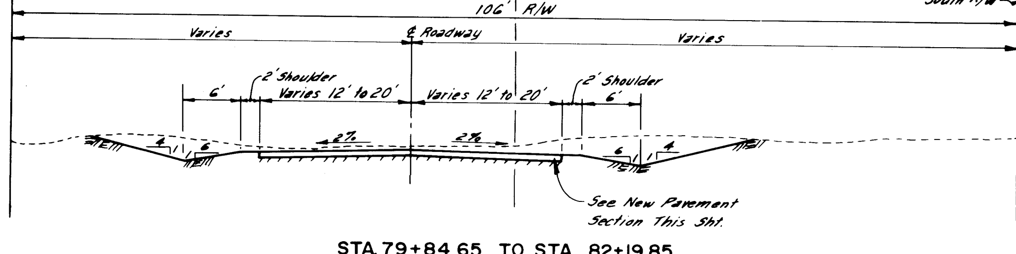
TYPICAL STREET SECTIONS SCALE: 1" = 10'
