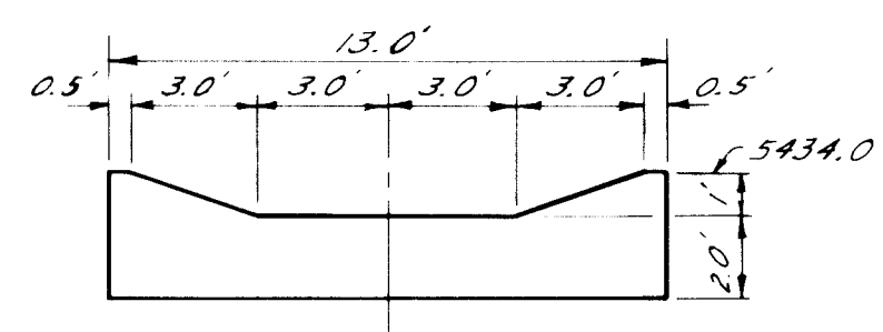
CUT-OFF WALL DETAIL SCALE: 1" = 5'
