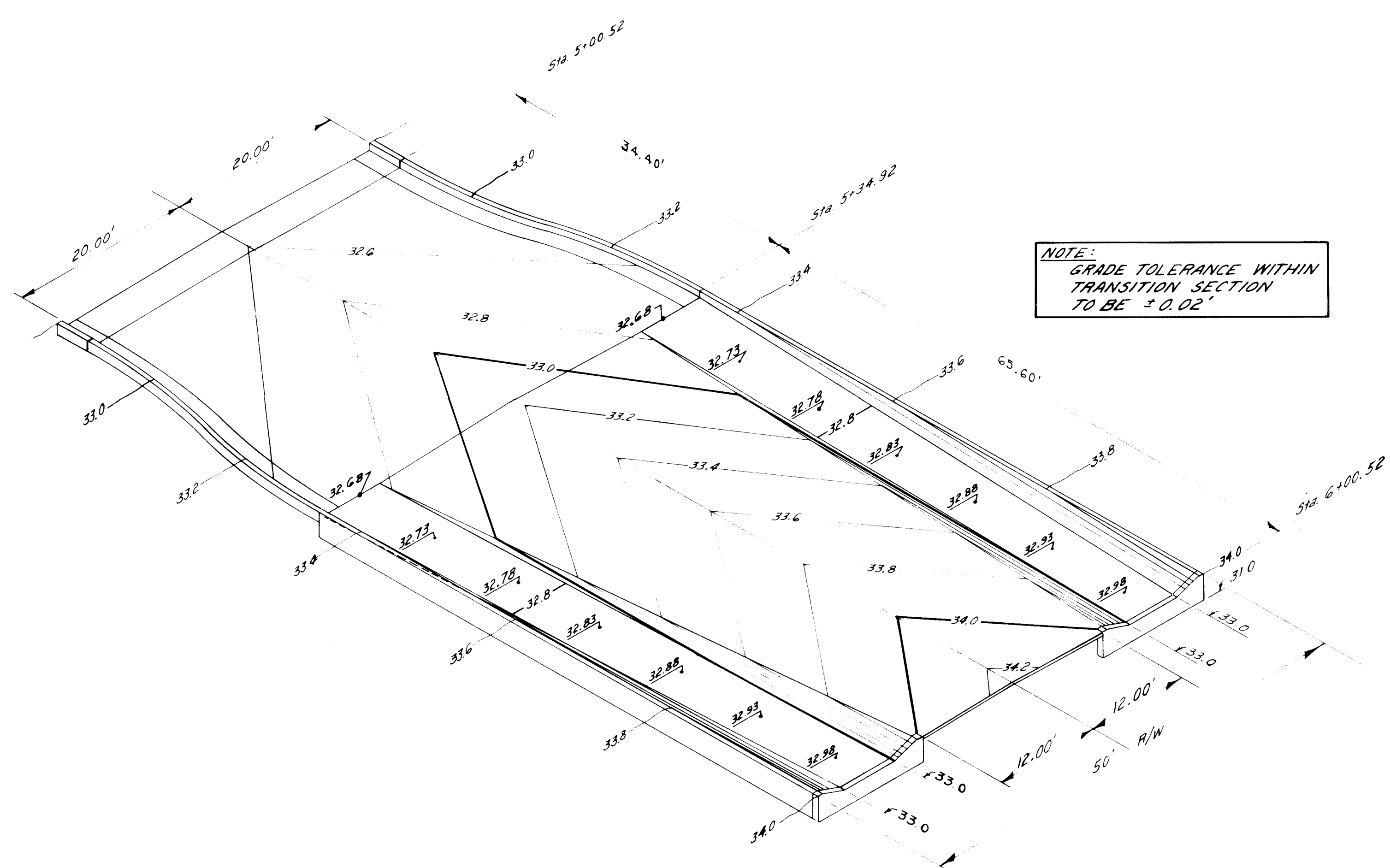
CHANNEL & ROAD TRANSITION SOMETRIC VIEW SCALE: 1" = 10'
