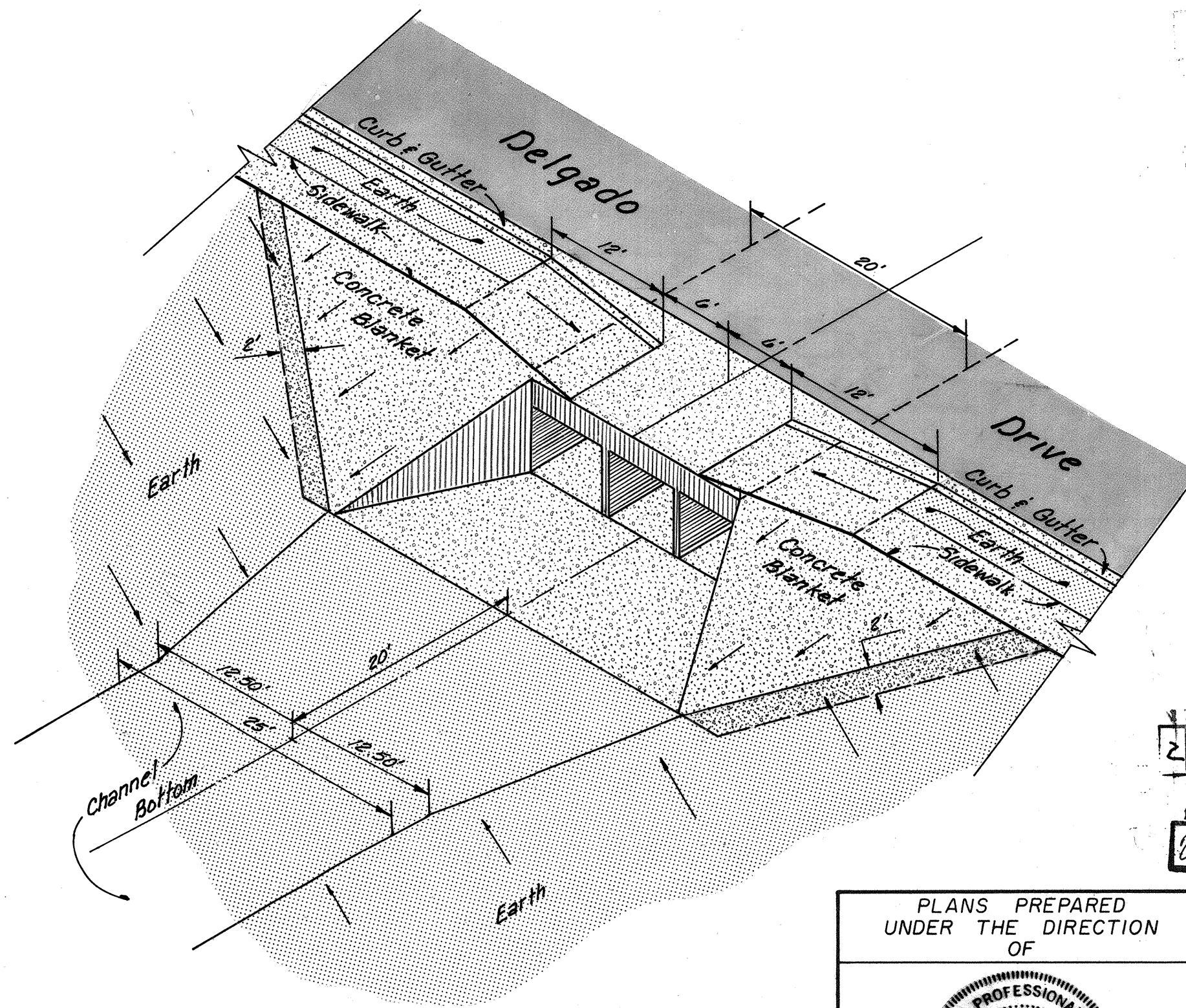
View Conc. Box Culvert Inlet
