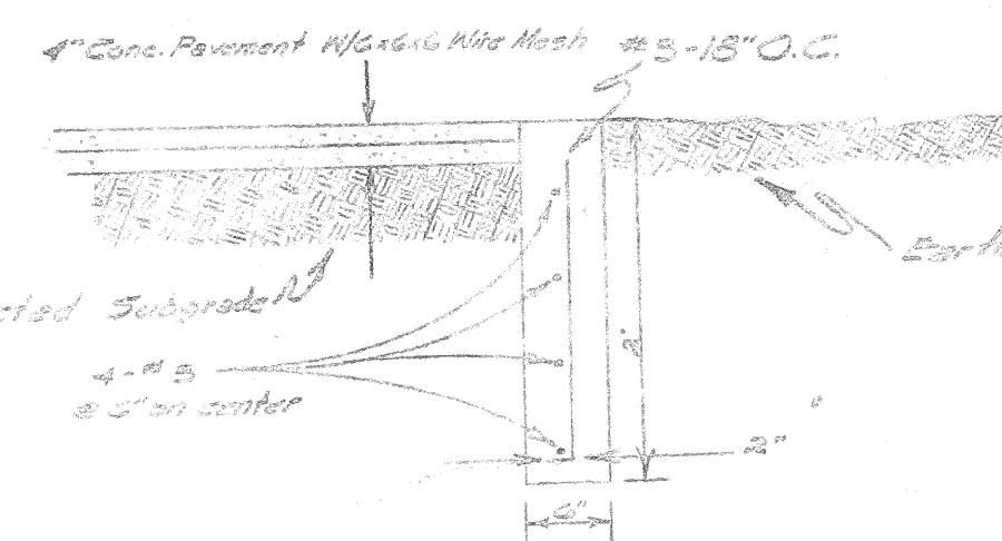
CUTOFF WALL DETAIL NO SCALE
