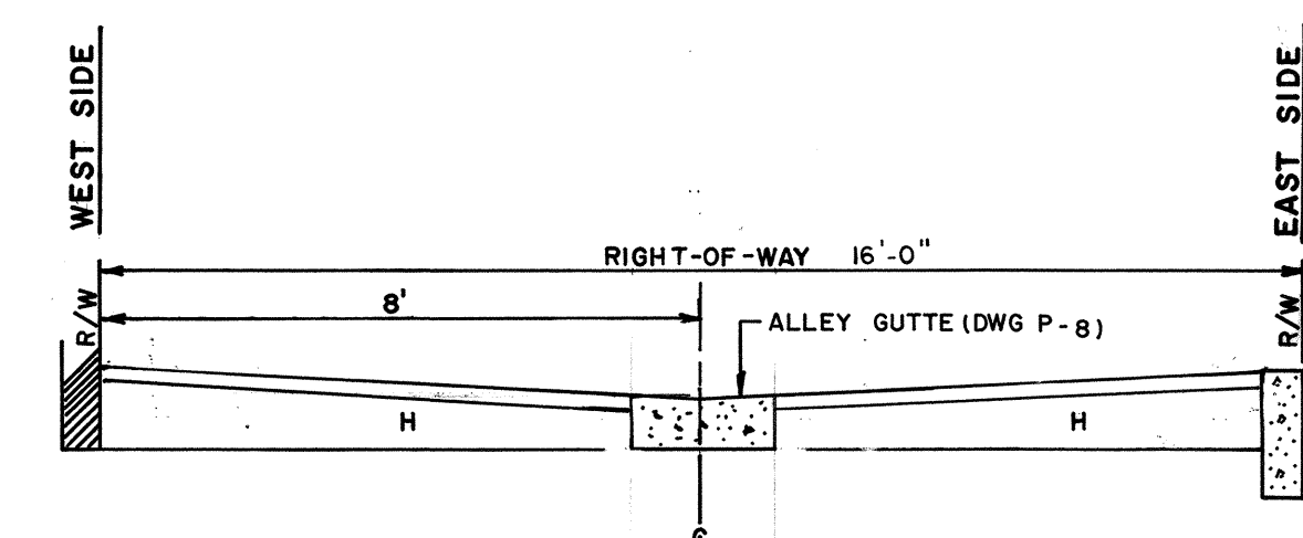
ALLEY SECTION DETAIL SECTION A-A (DWG. P-6)
