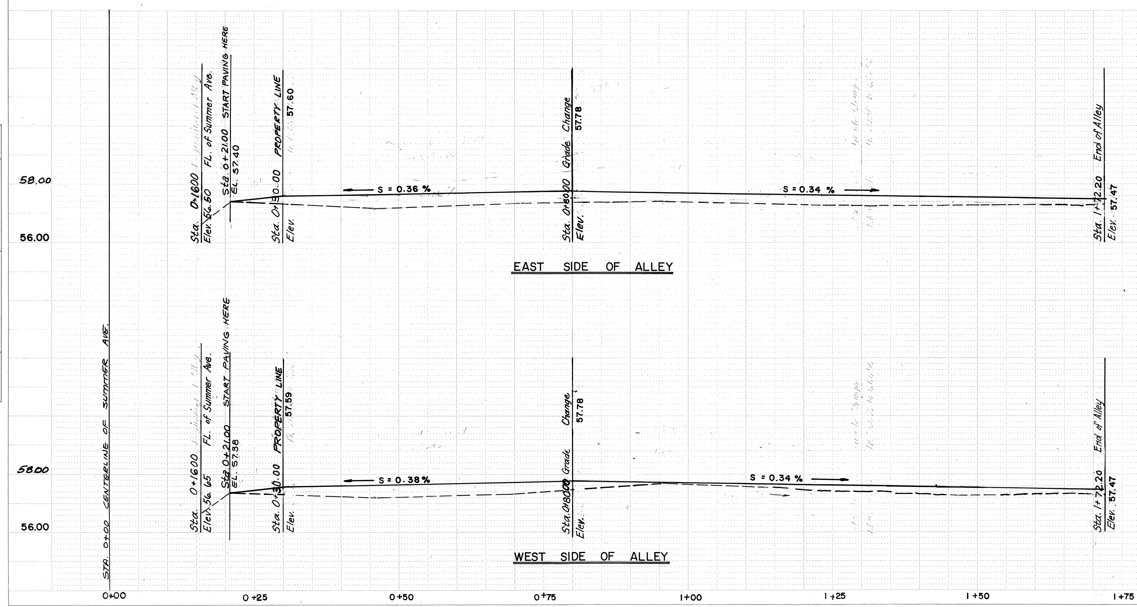
PLATE 1 SINGLE PLAN - PROFILE - DOTTED CHARLES BRUSHING COMPANY MADE IN U.S.A.
