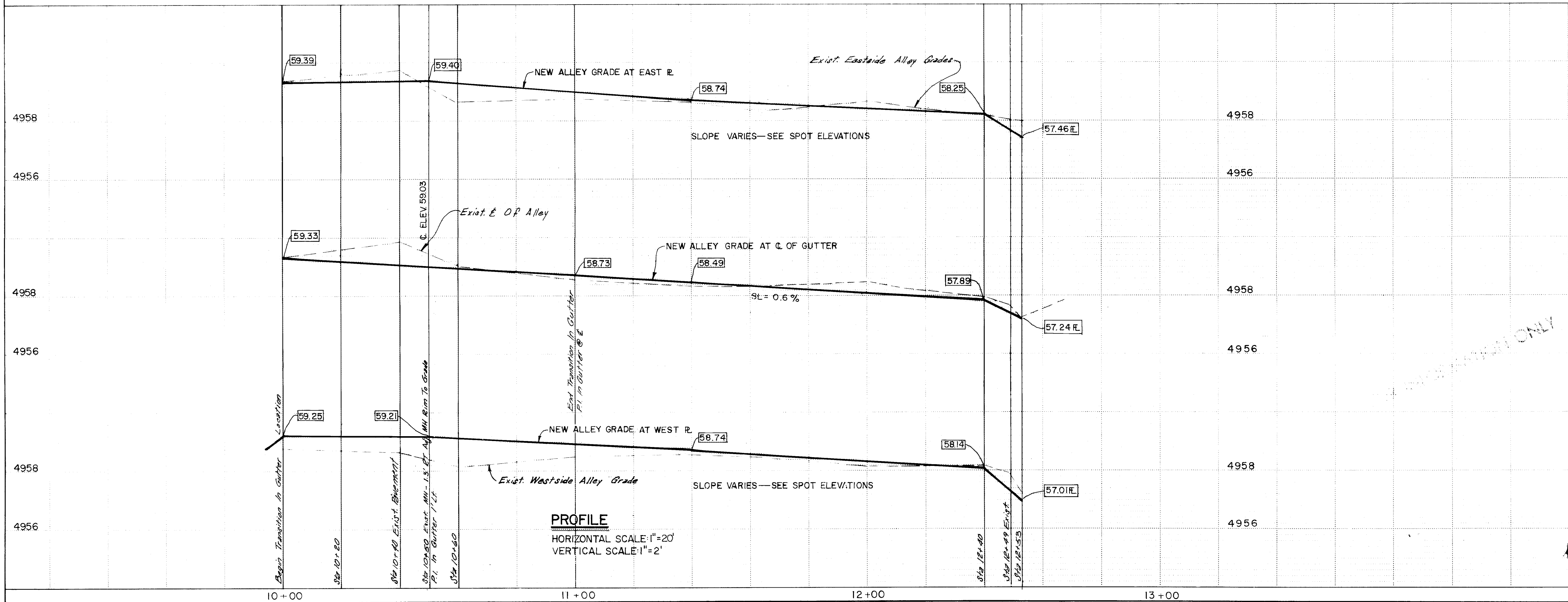
ALLEY GRADES
