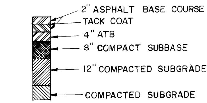
TYPICAL PAVEMENT SECTION
