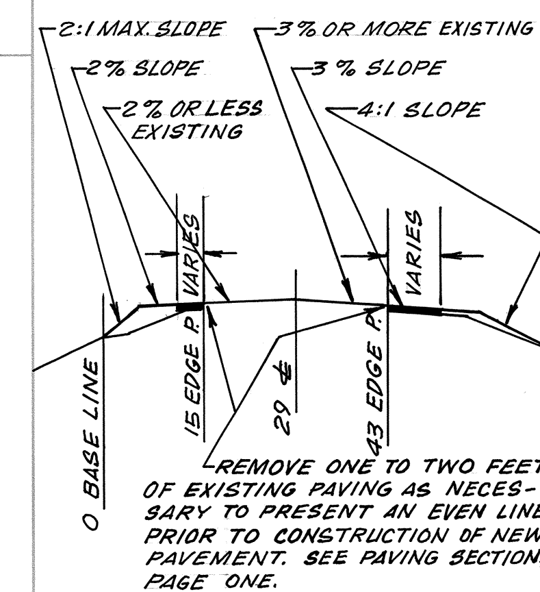
TYPICAL STREET SECTION NO SCALE
