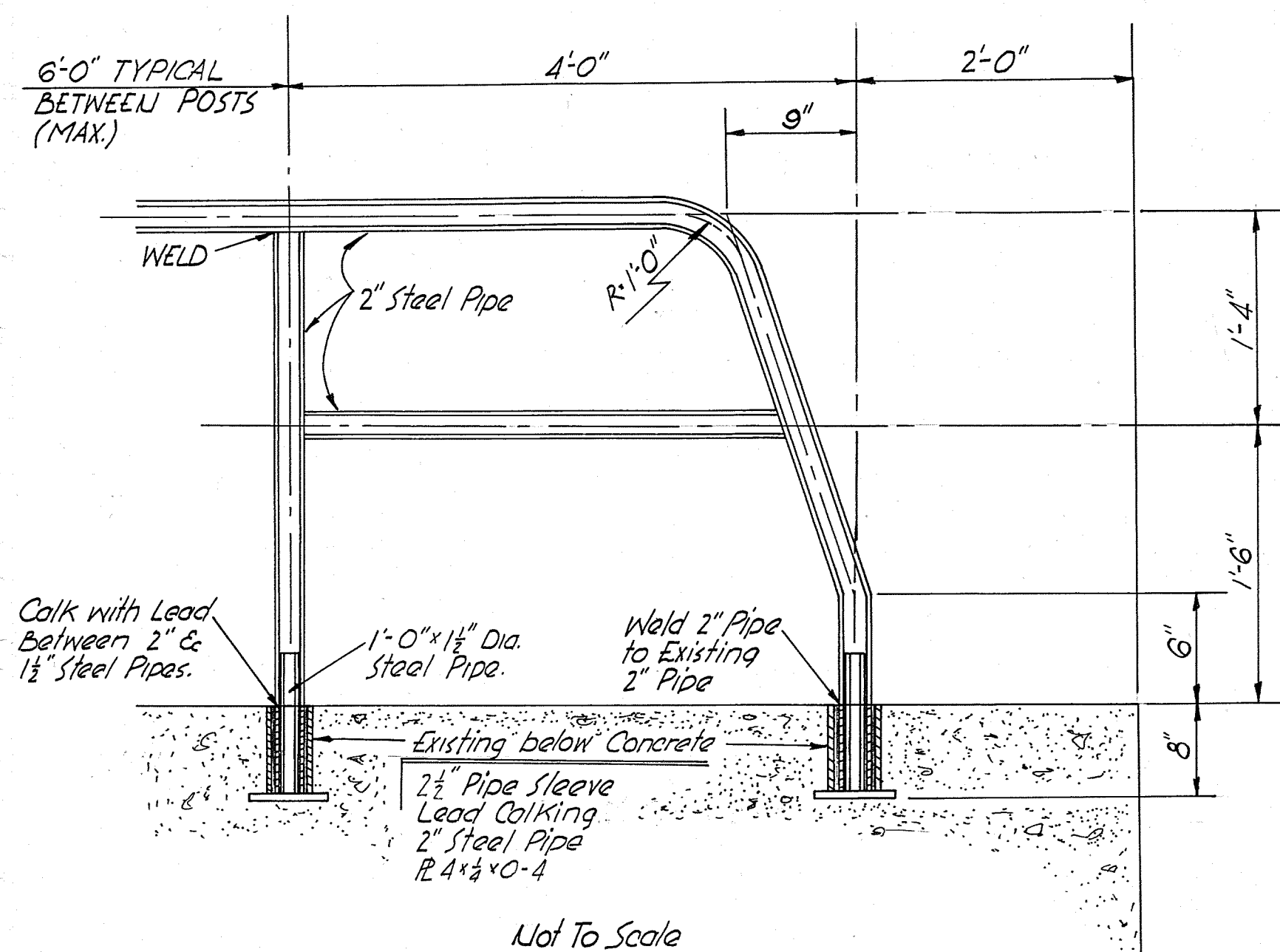
Not To Scale A-A HANDRAIL DETAIL
