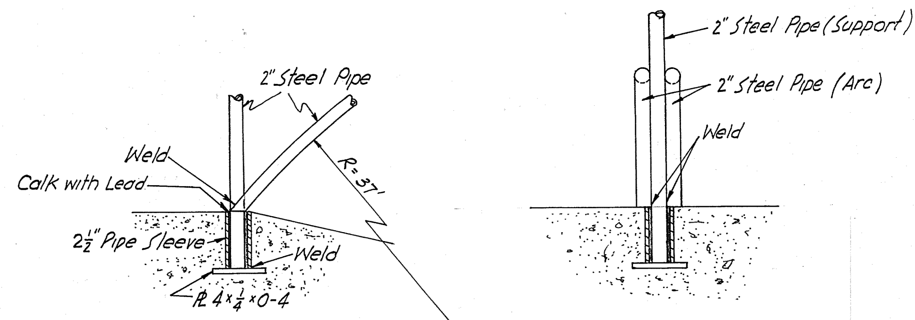
Not To Scale SECTION C ARCH & SUPPORT HANDRAIL DETAIL
