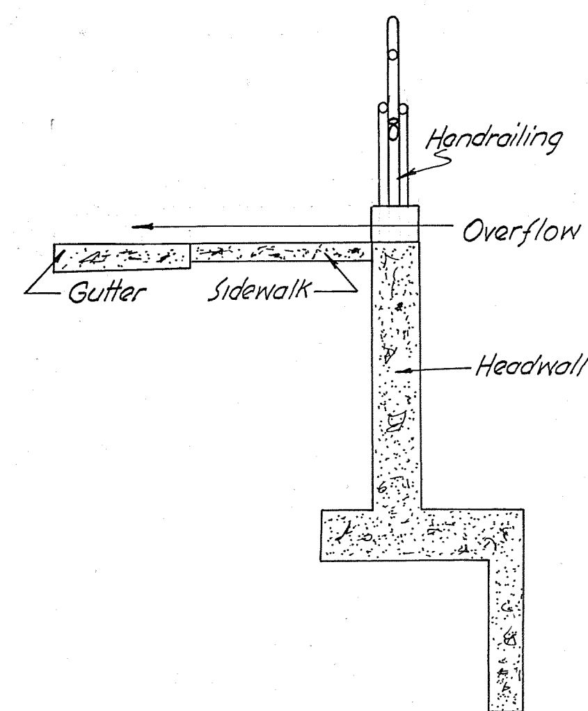
Not To Scale B-B WEST HEADWALL DETAIL
