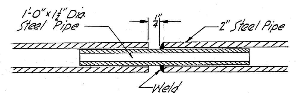
SECTION D HANDRAIL EXTENSION JOINT Not To Scale
