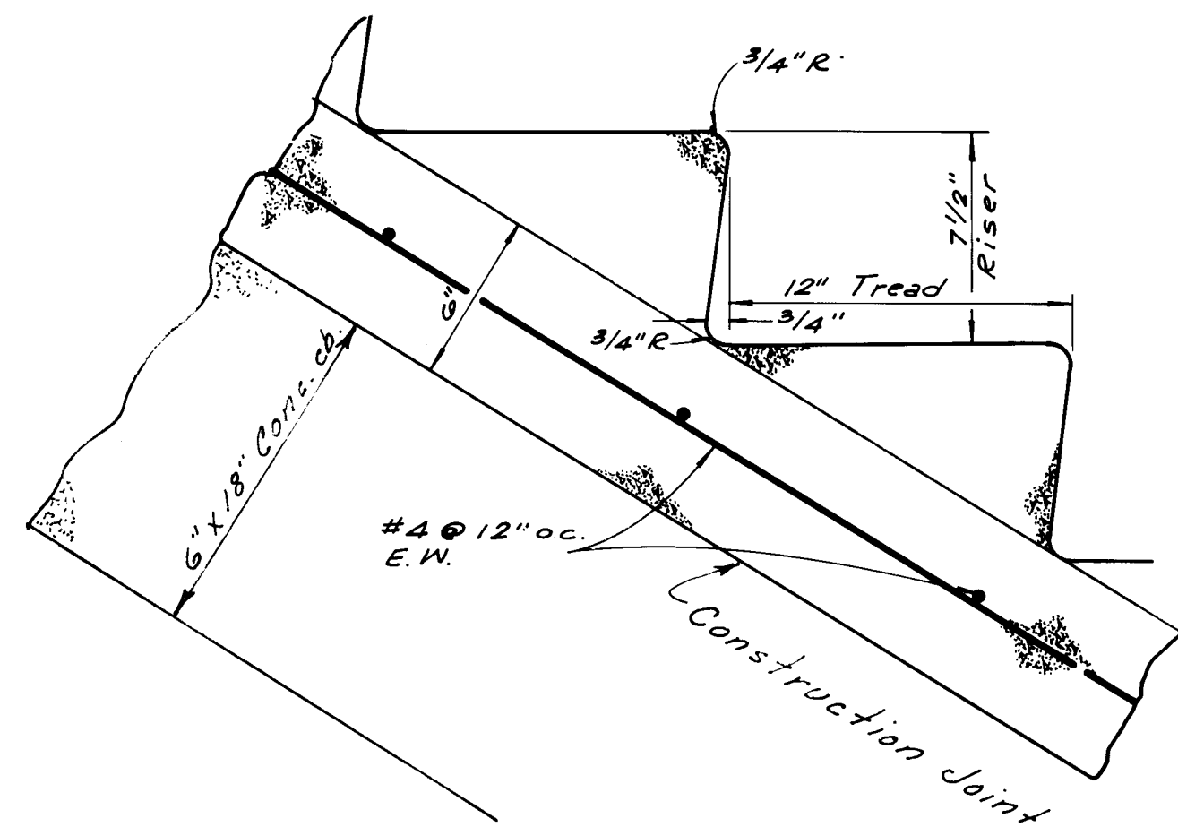
STAIR DETAIL
