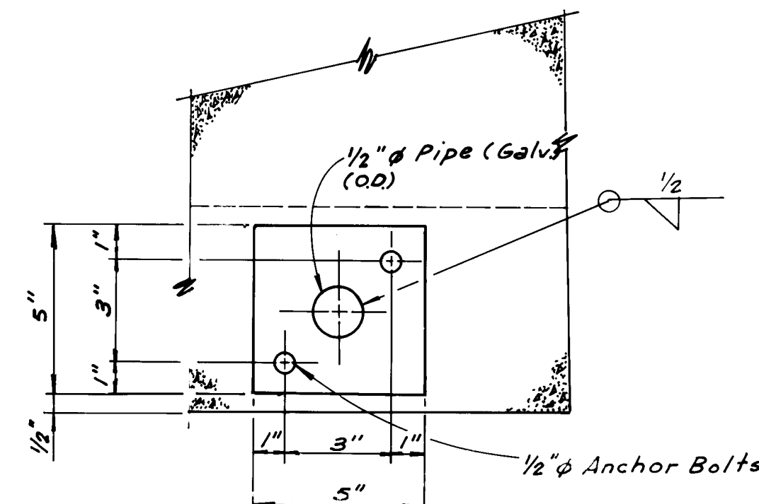
PLATE DETAILS SCALE: 1/4" = 1'-0"
