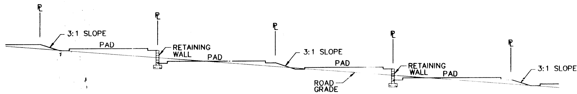
SECTION O-O TYPICAL PAD LAYOUT N.T.S.
