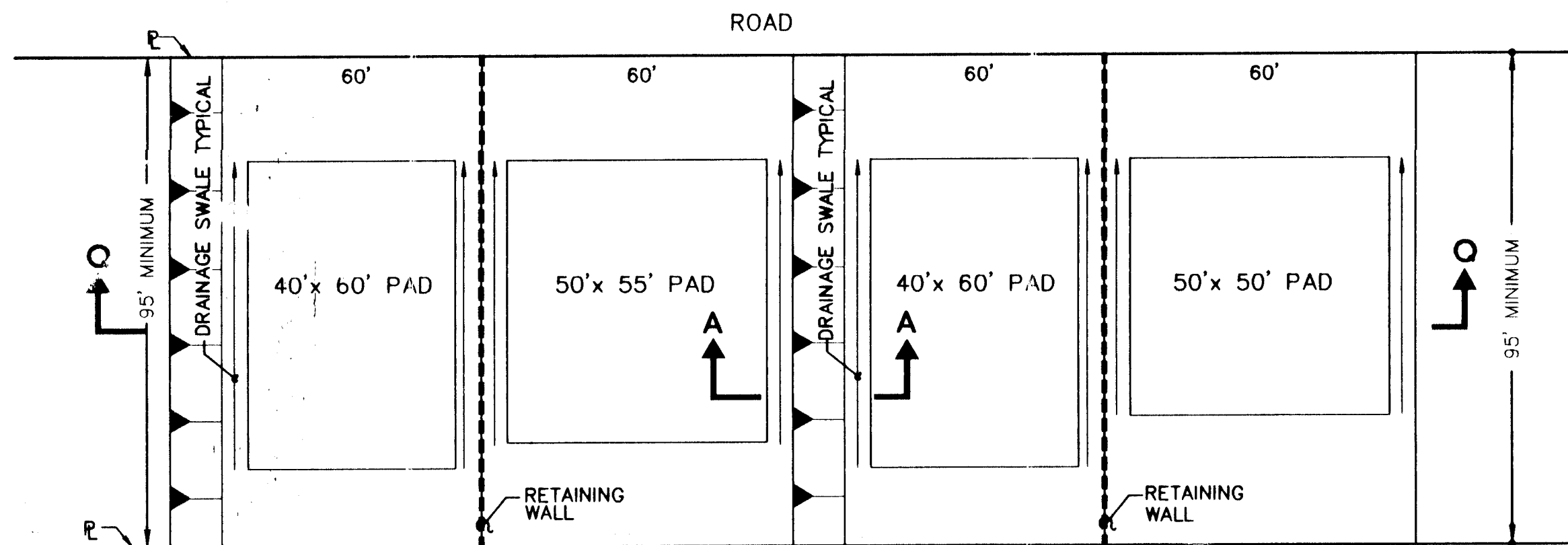
TYPICAL PAD LAYOUT N.T.S.
