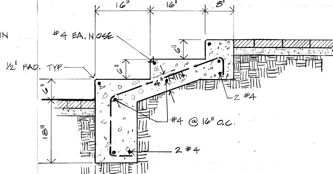
2 SECTION THROUGH STAGE STEPS SCALE 3/4" = 1'-0"
