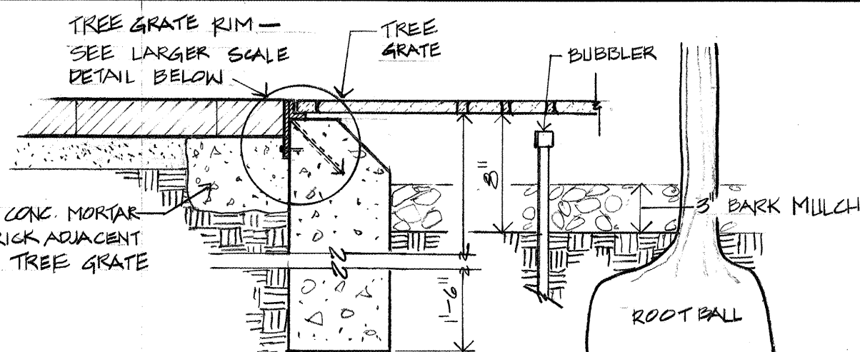
11 SECTION 'C-C' TREE GRATE PLAN NO SCALE
