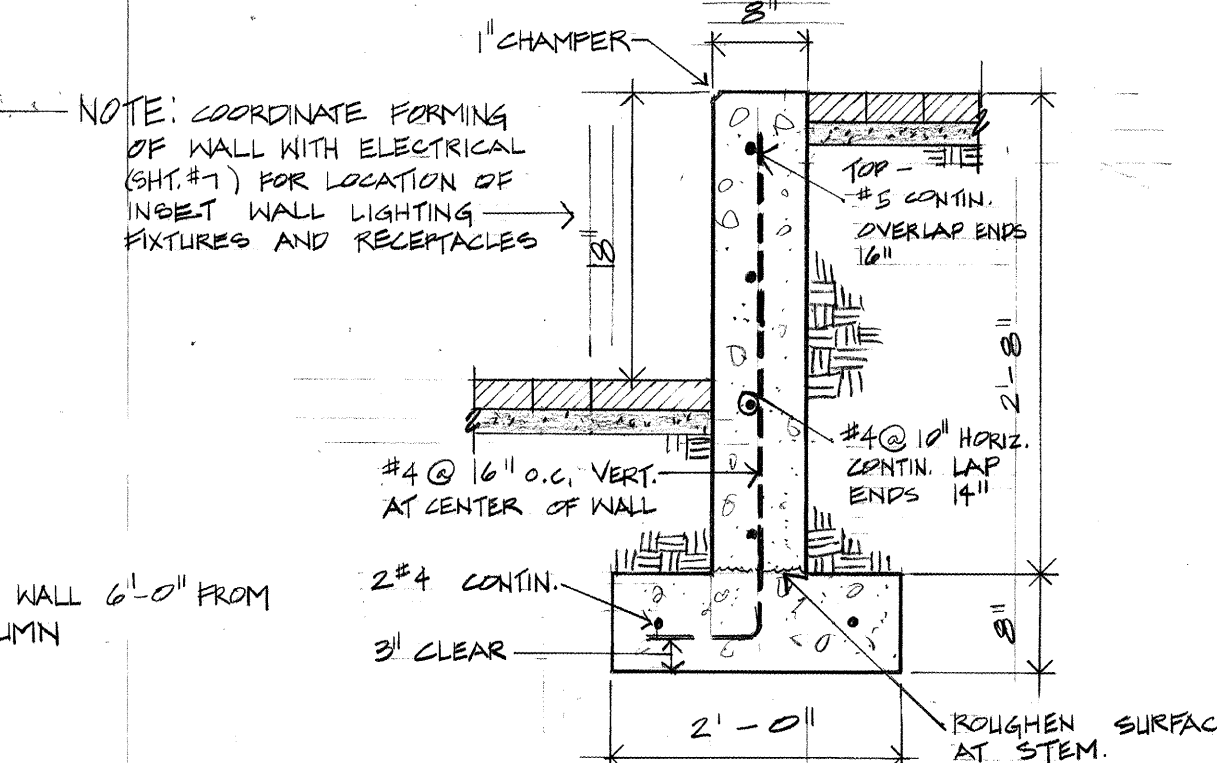
1 SECTION 'B-B' THROUGH STAGE WALL SCALE = N.T.S.
