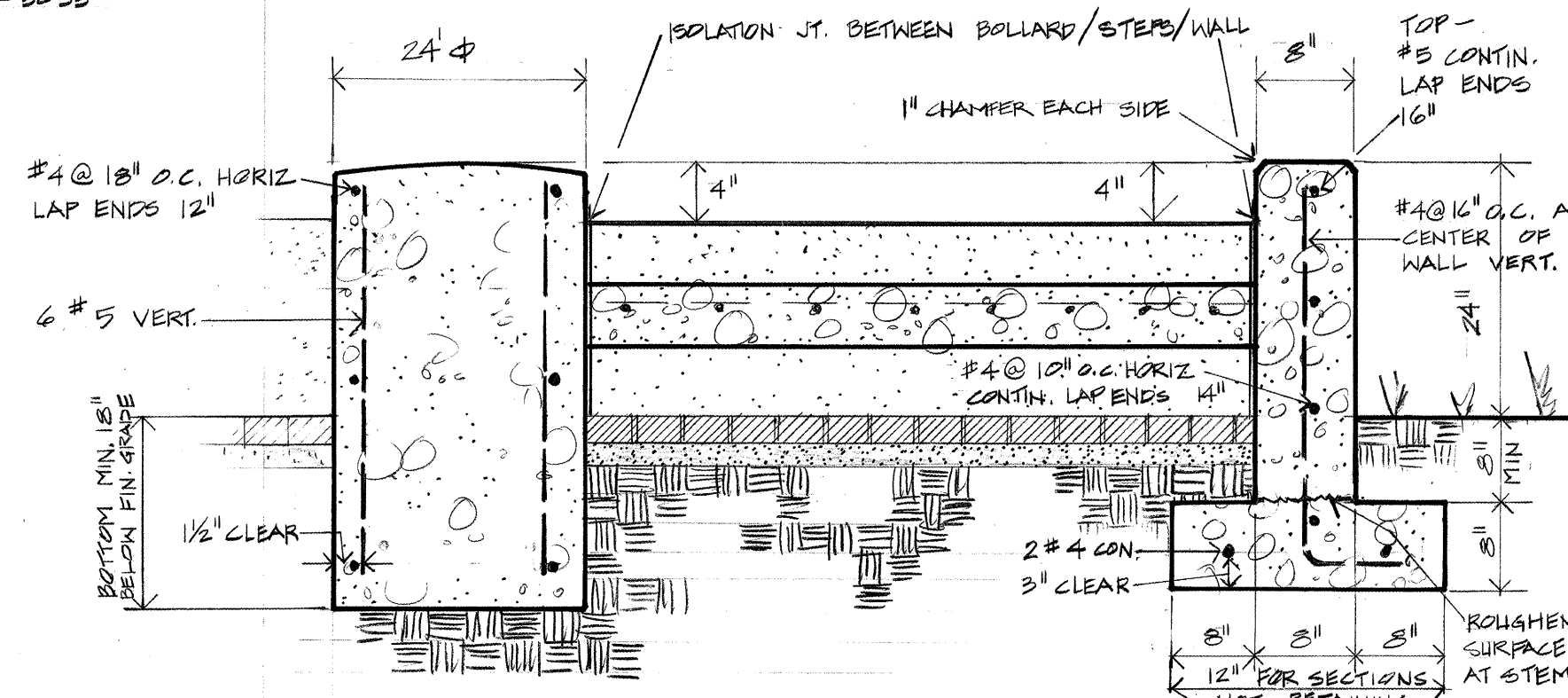
1 SECTION 'A-A' THROUGH BOLLARD & STAGE STEPS SCALE 3/4" = 1'-0"
