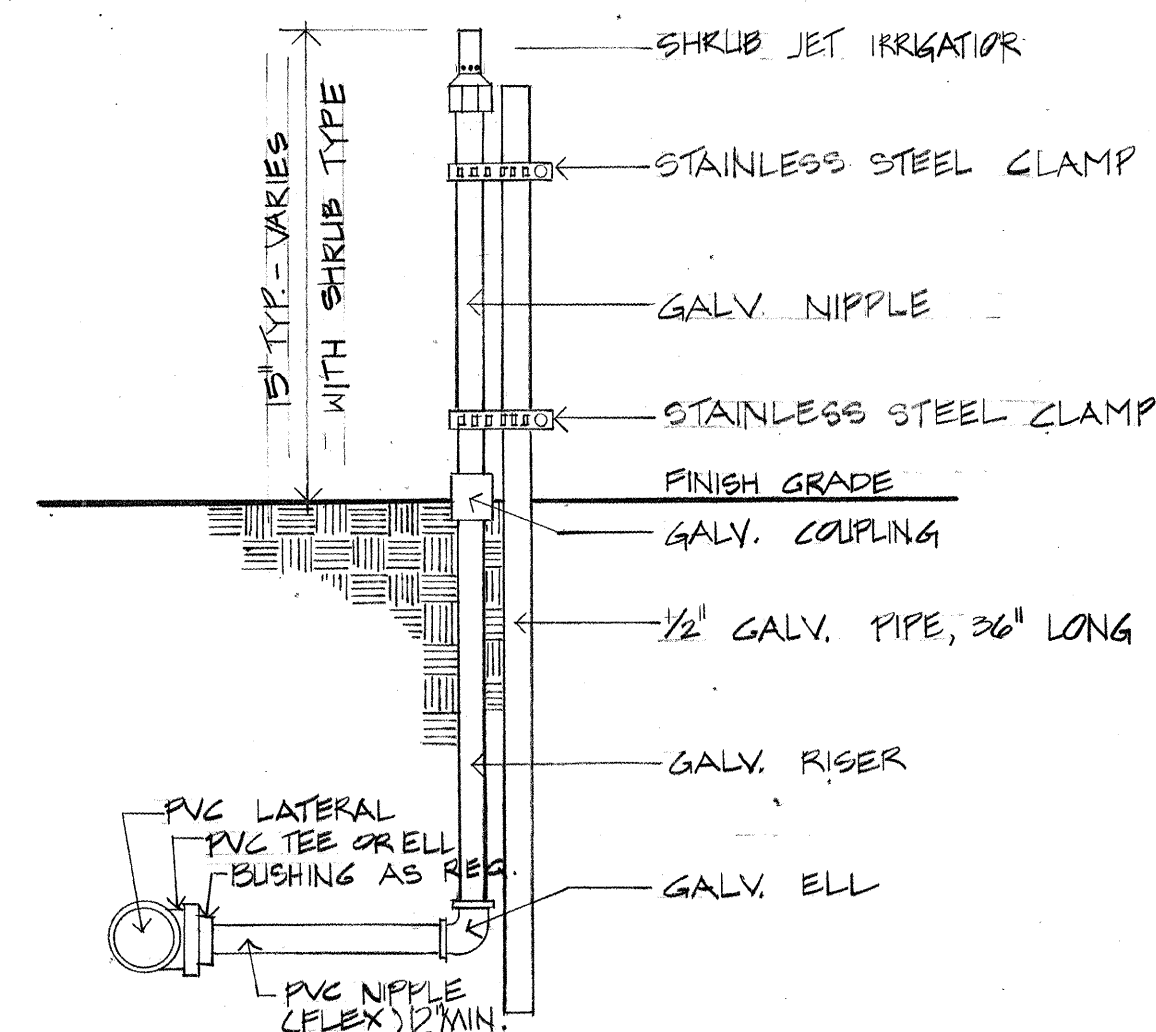
2 SHRUB RISER DETAIL 6
