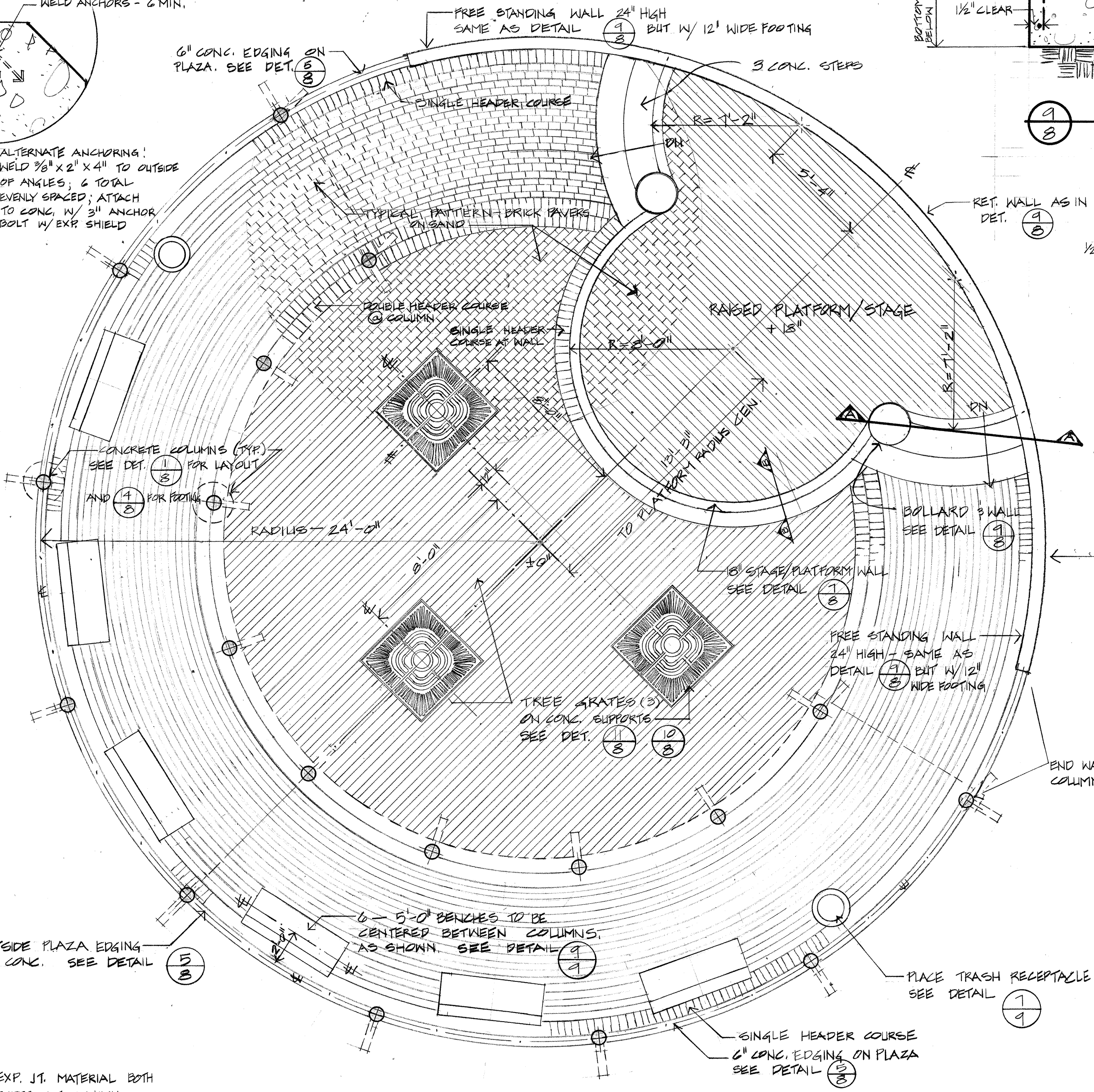
12 TREE GRATE PLAN NO SCALE
