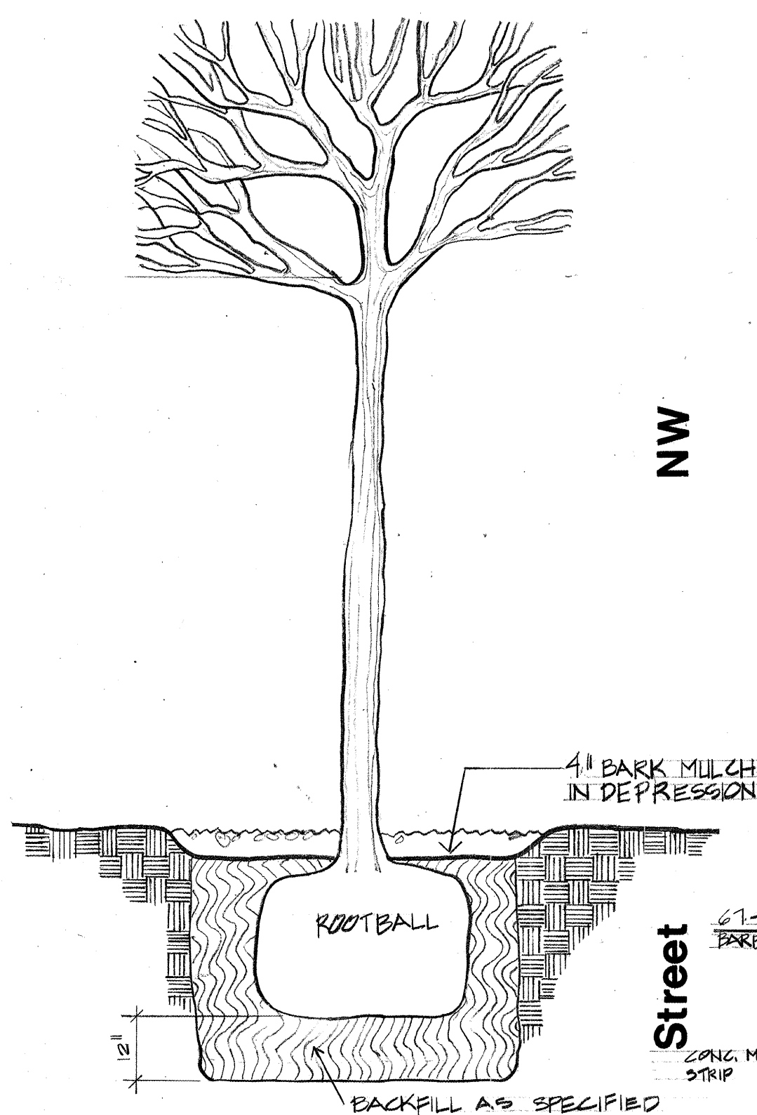
TREE PLANTING DETAIL (TYPICAL IN NON-LAWN AREA) N.T.S.
