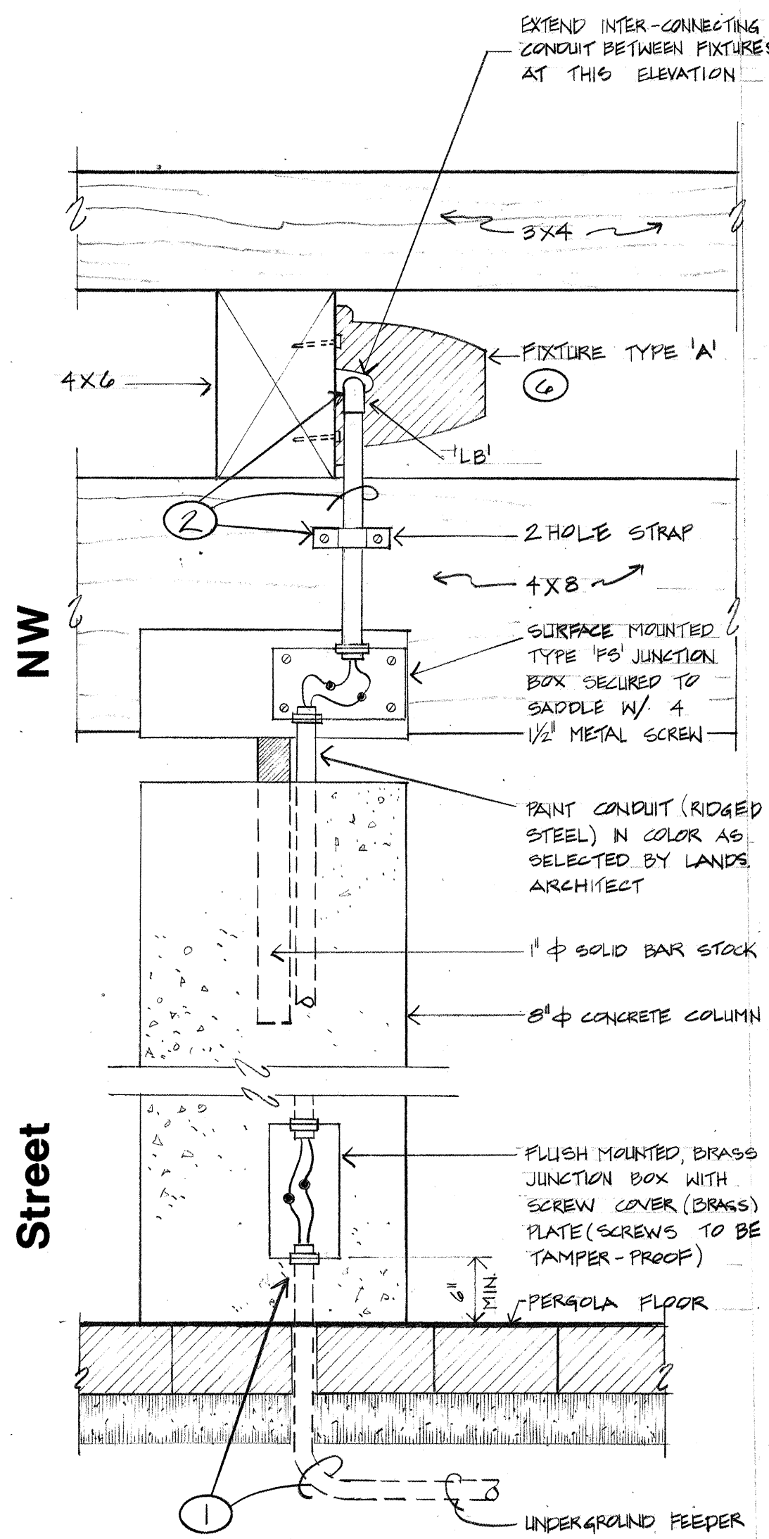
TYPE 'A' FIXTURE MOUNTING DETAIL NO SCALE
