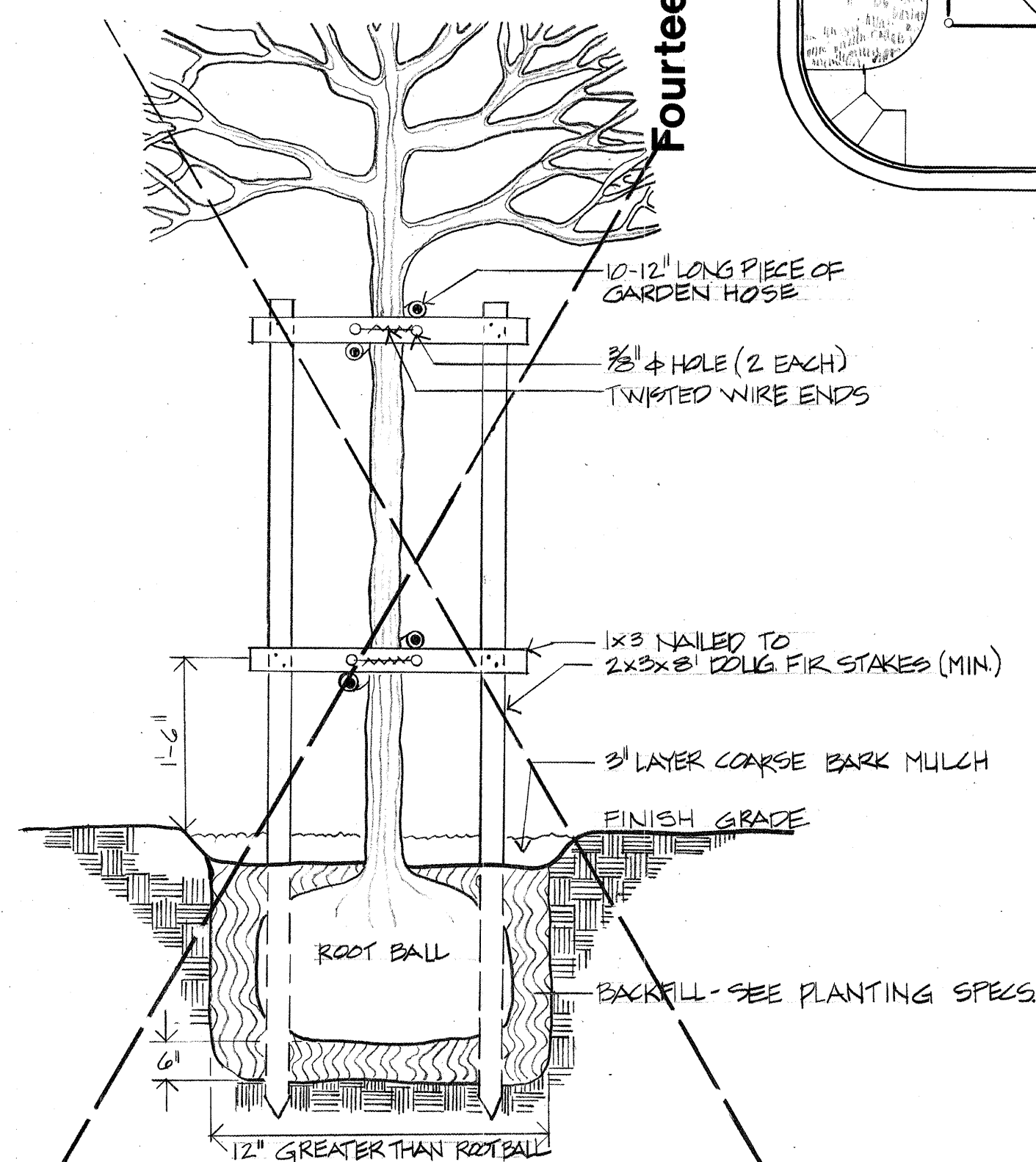
TREE STAKING AND PLANTING DETAIL NO SCALE (THIS DETAIL NOT REQUIRED THIS PROJECT)
