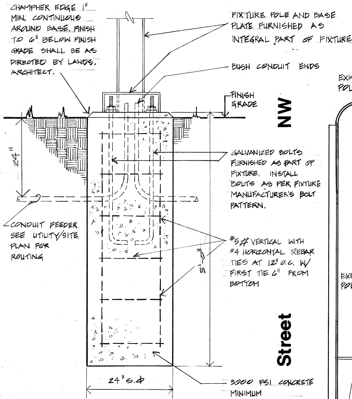
FIXTURE TYPES 'C' & 'D' MOUNTING DETAIL NO SCALE
