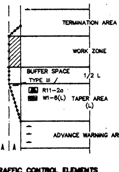
TRAFFIC CONTROL ELEMENTS
