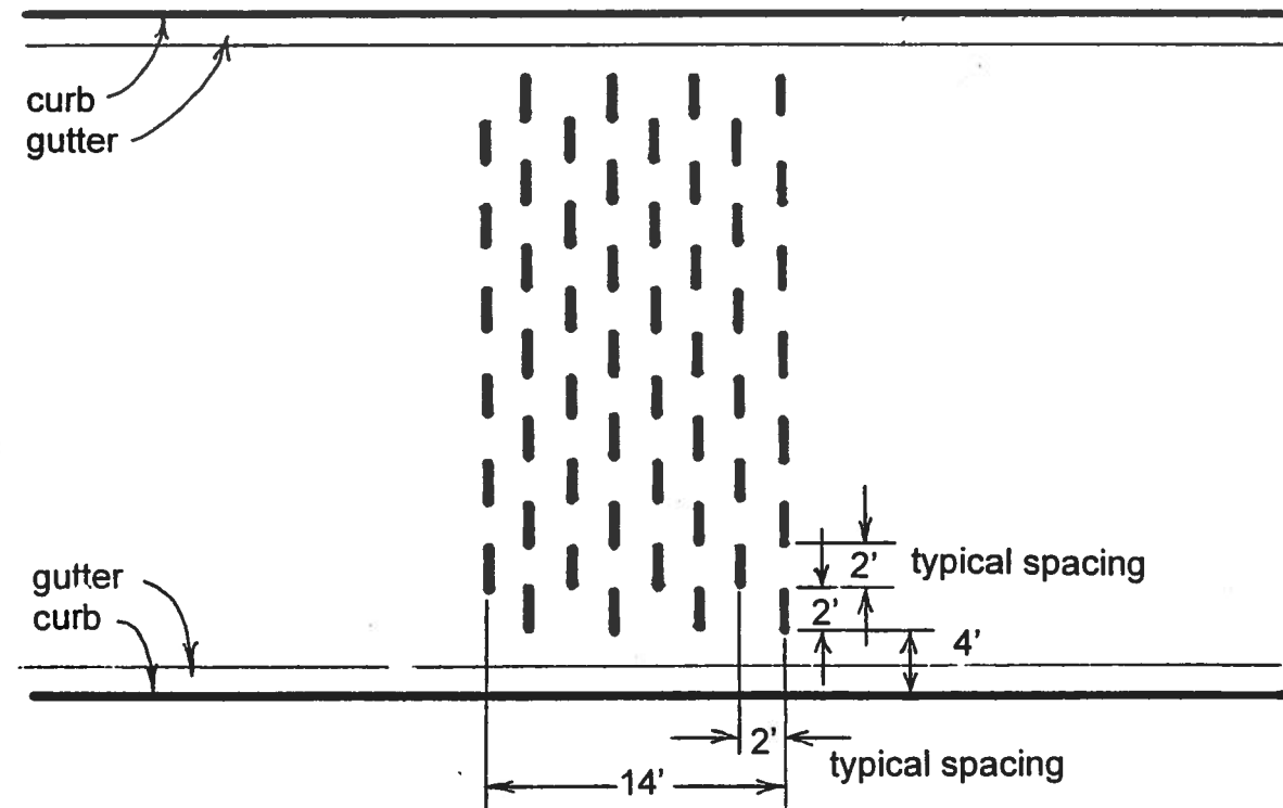
Plan view 1" = 10'
