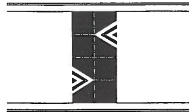
MARKING PLAN
