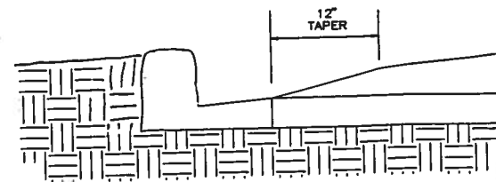
CURB TREATMENT
