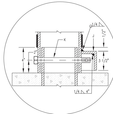
DETAIL B SECTION A-A
