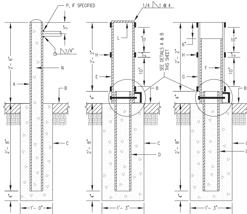
STATIONARY POST
