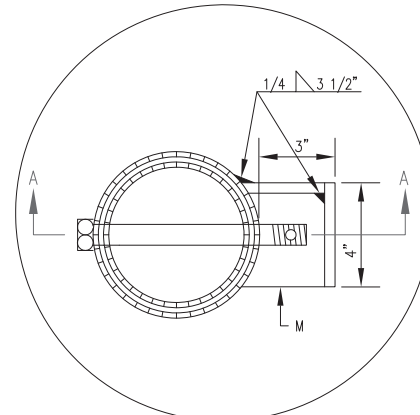
DETAIL A PLAN
