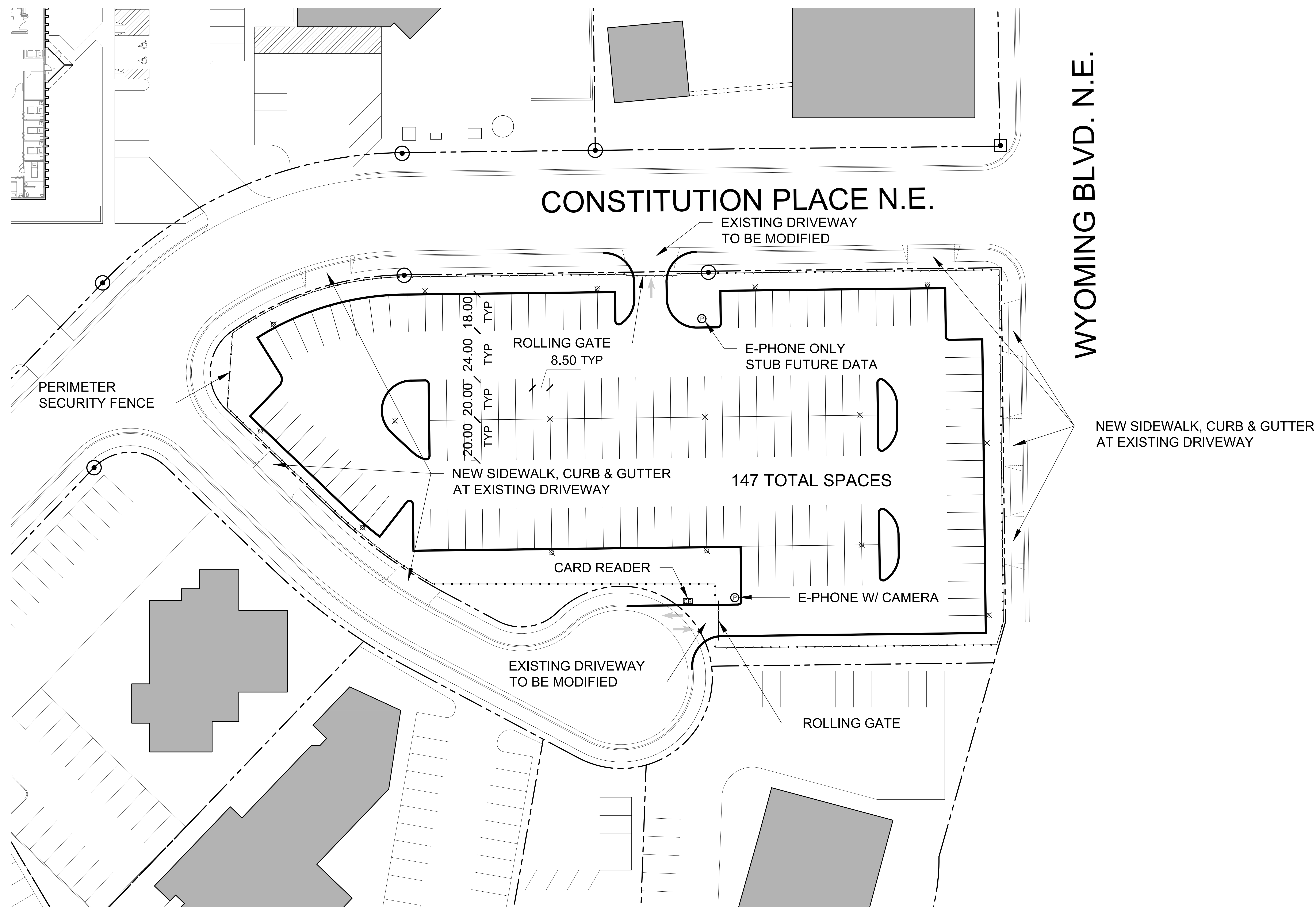
A SITE PLAN (OPTION A) 1" = 20'-0"
