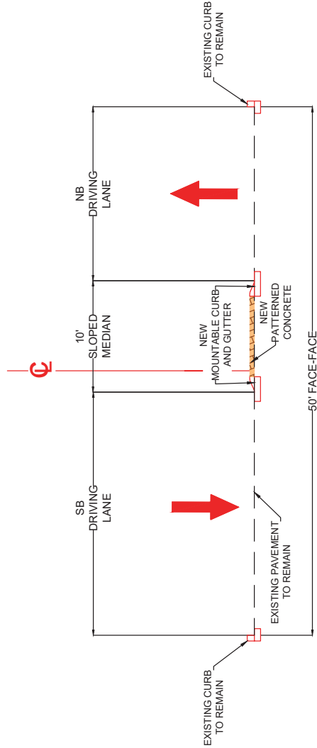
CARLISLE BLVD - PROPOSED SECTION AA
