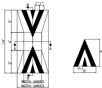
SPEED CUSHION STRIPING LAYOUT
