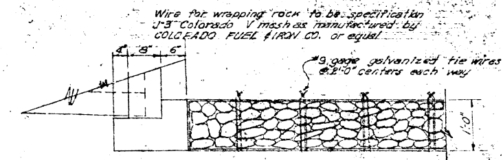
WIRE ENCLOSED RIPRAP NOT TO SCALE.
