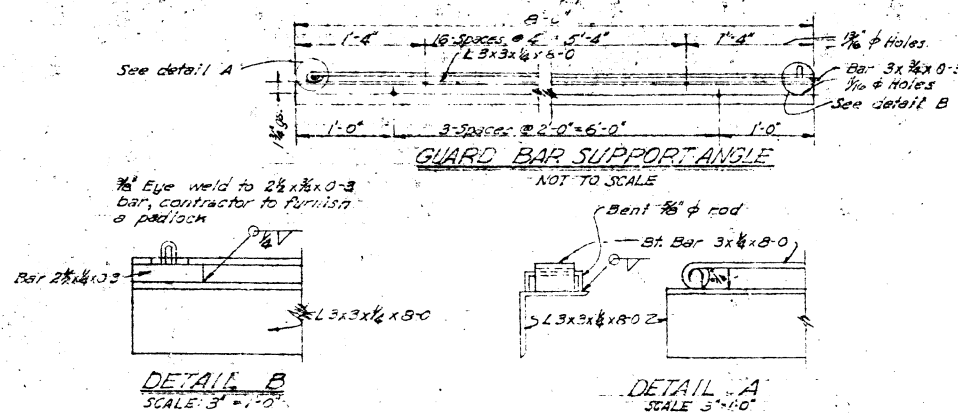
HEADWALL DETAILS
