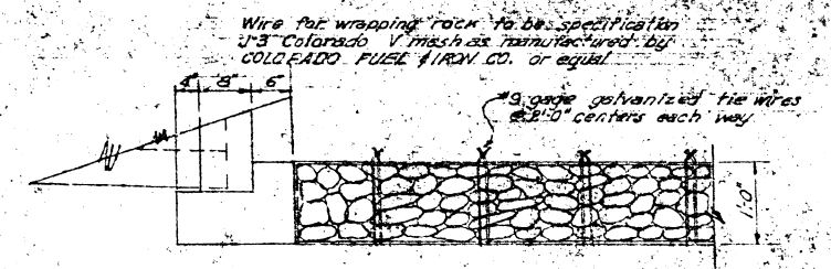
WIRE ENCLOSED RIPRAP NOT TO SCALE.
