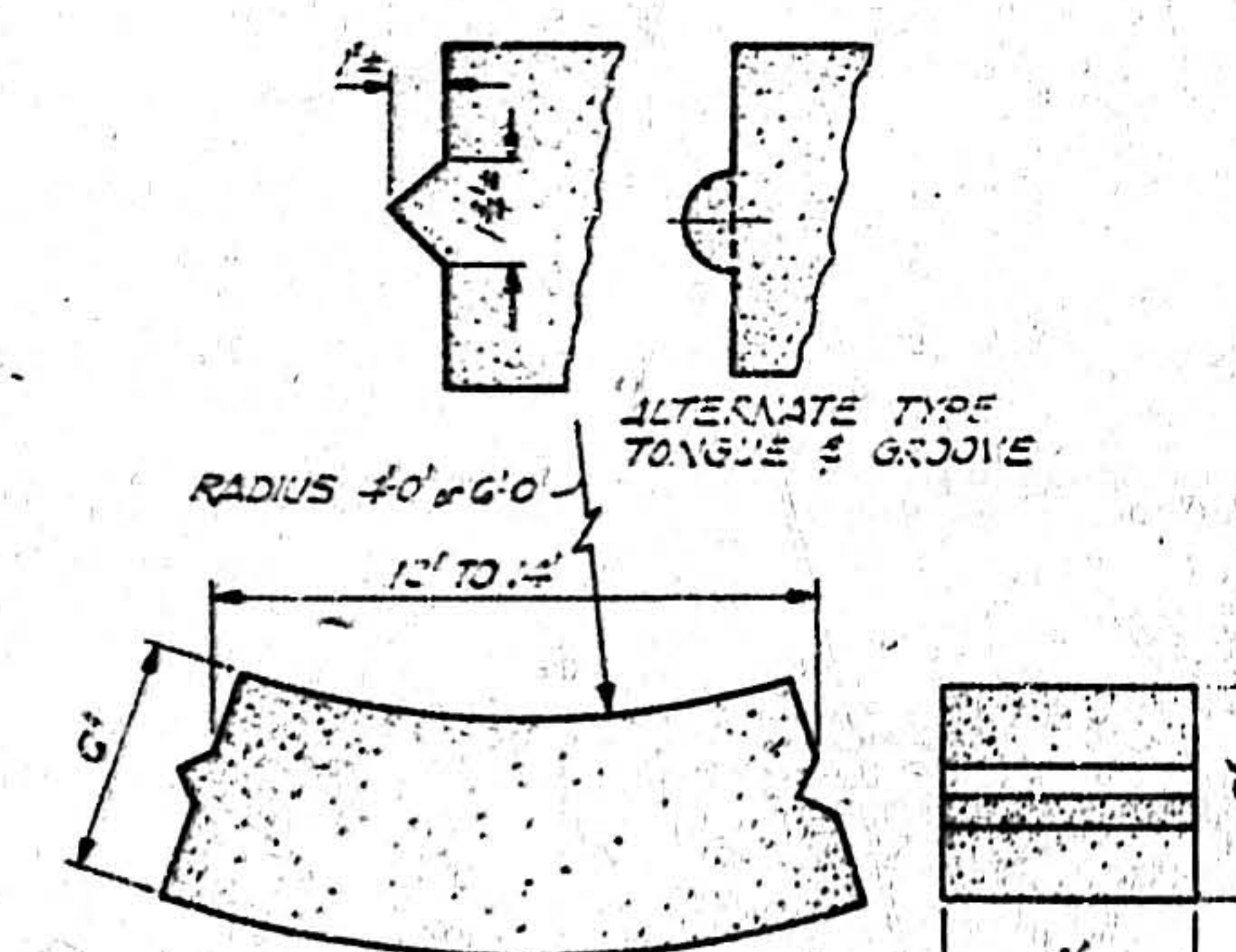
TYPICAL DETAIL OF CONCRETE BLOCK
