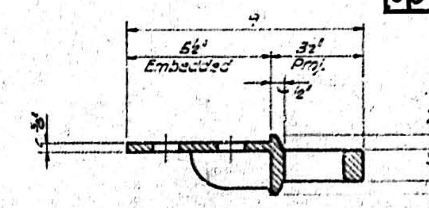
SECTION
