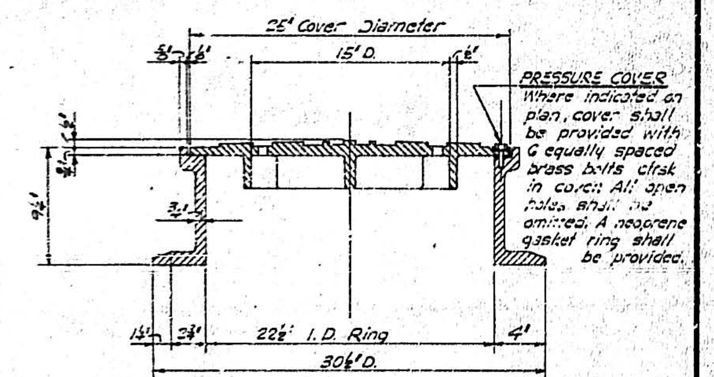
SECTION
