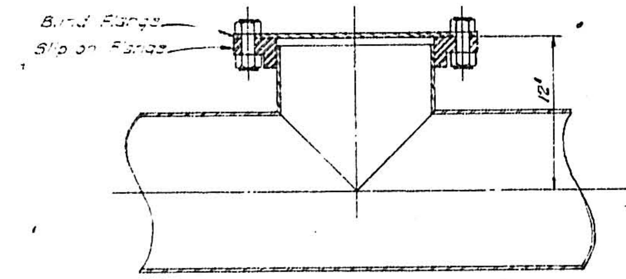
SECTION
