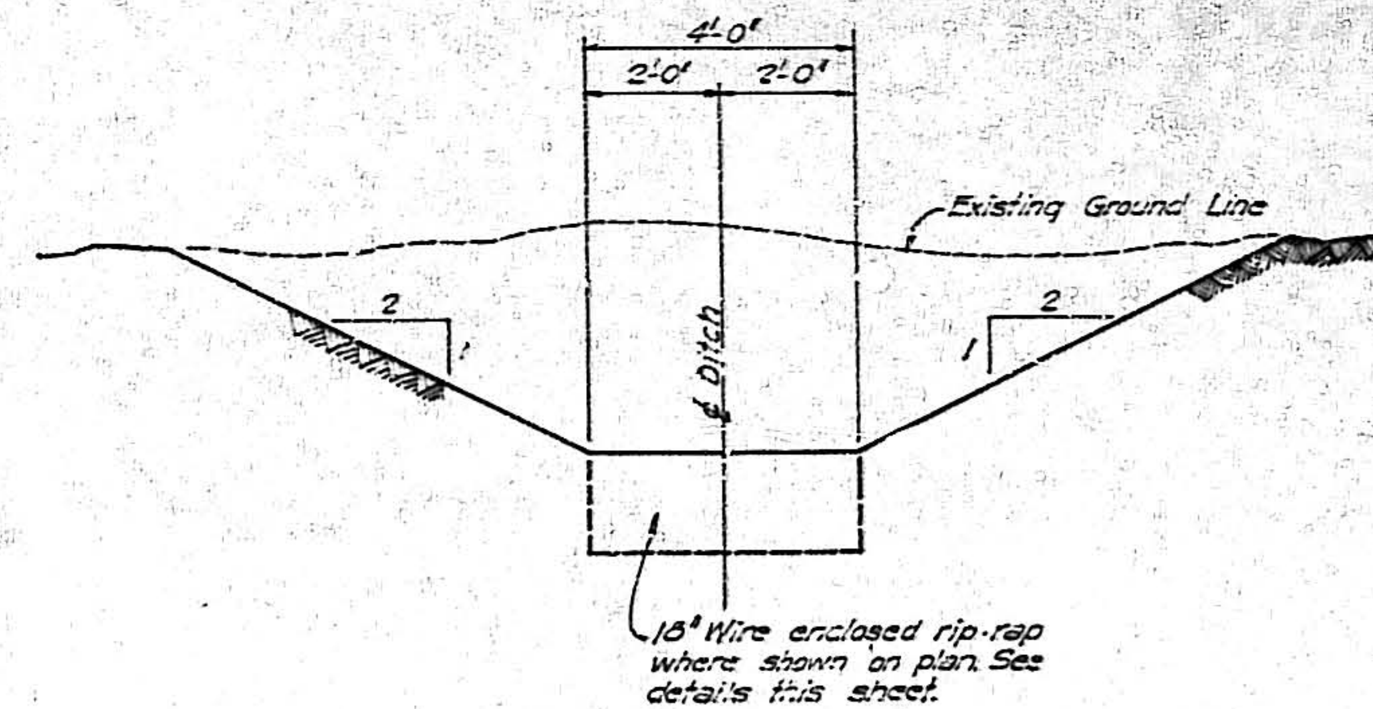
TYPICAL OPEN DITCH SECTION SCALE 3/4" = 1'-0"
