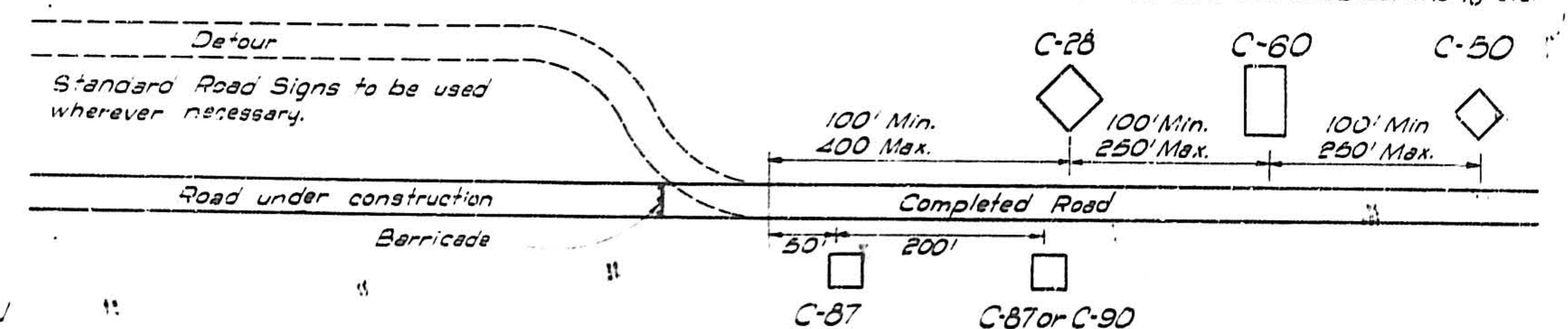
TYPICAL SIGN LAYOUT FOR DETOUR
