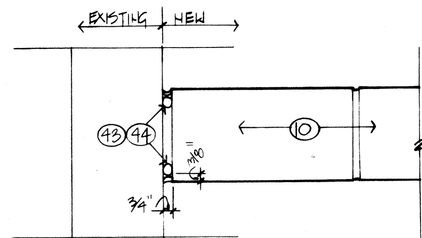
11 Expansion Joint 1 1/2" = 1' - 0"
