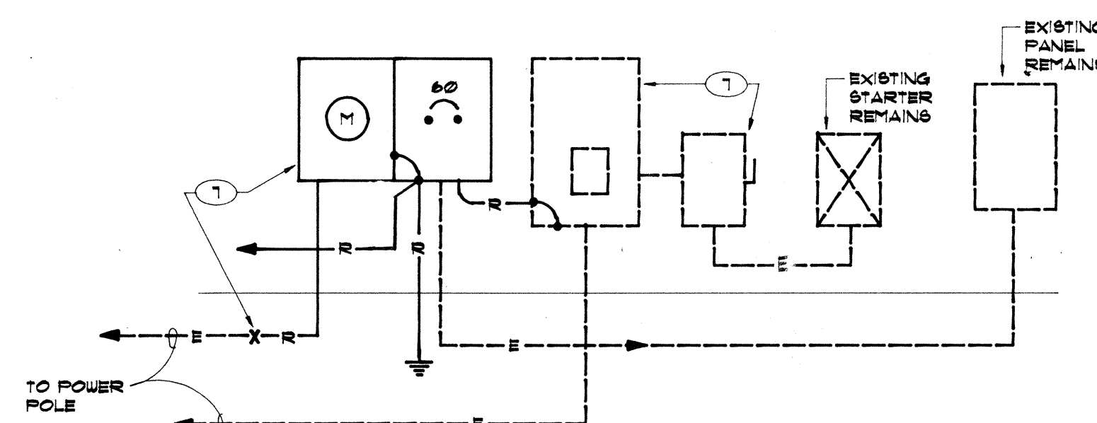
NTB POWER RISER DIAGRAM - DEMOLITION
