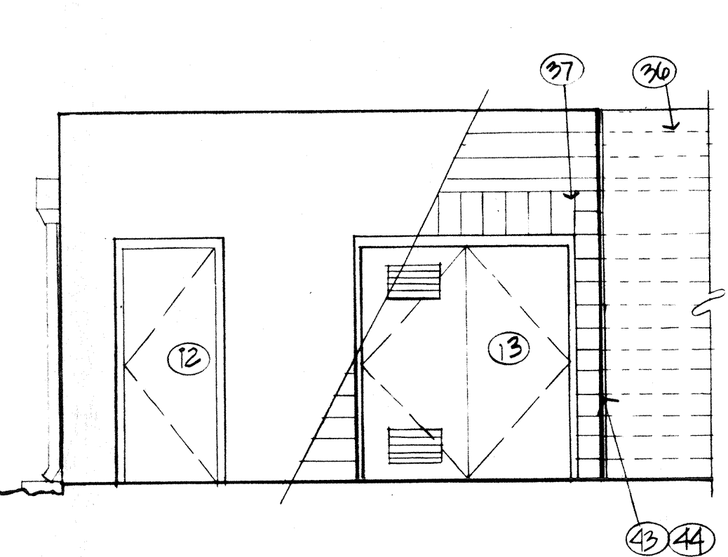
5 North Elevation 1/4" = 1' - 0"
