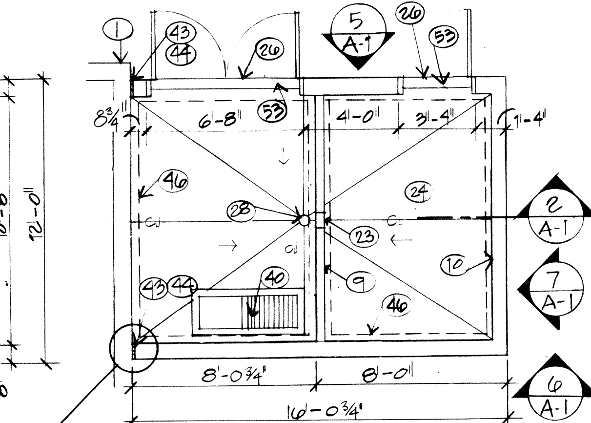
3 Floor/Foundation Plan 1/4" = 1' - 0"
