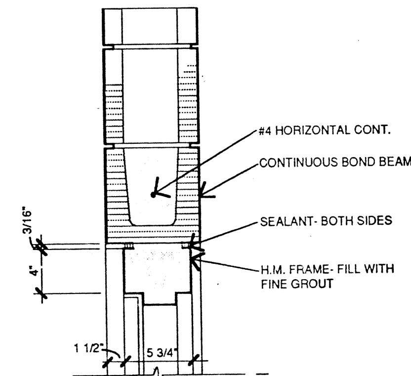
8 Head (Jamb @ dbl. dr. sim.) 1 - 1/2" = 1' - 0"
