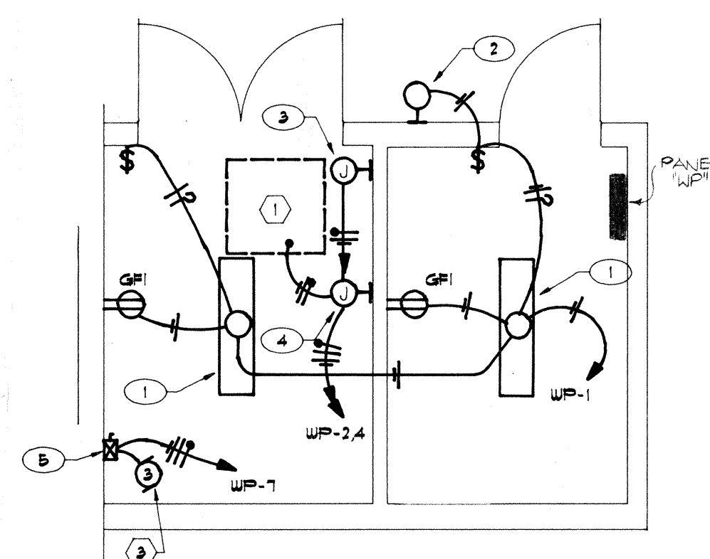
1/4"=1'-0" ELECTRICAL PLAN
