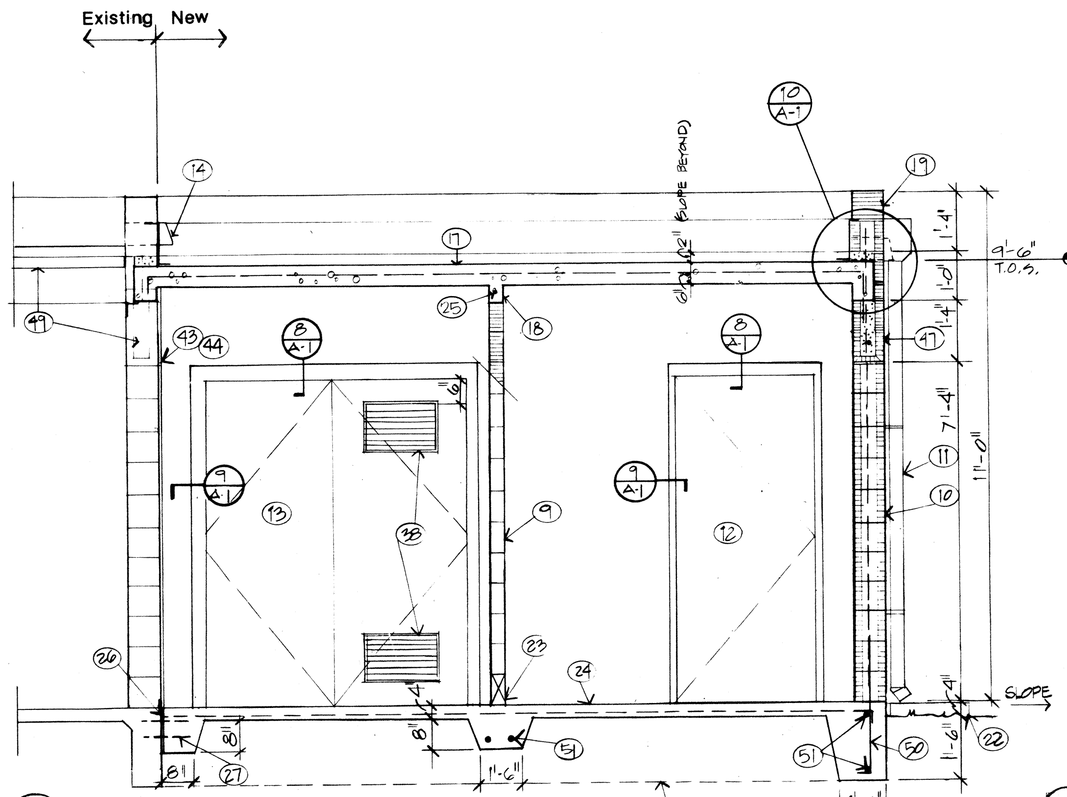
2 Building Section 1/2" = 1' - 0"
