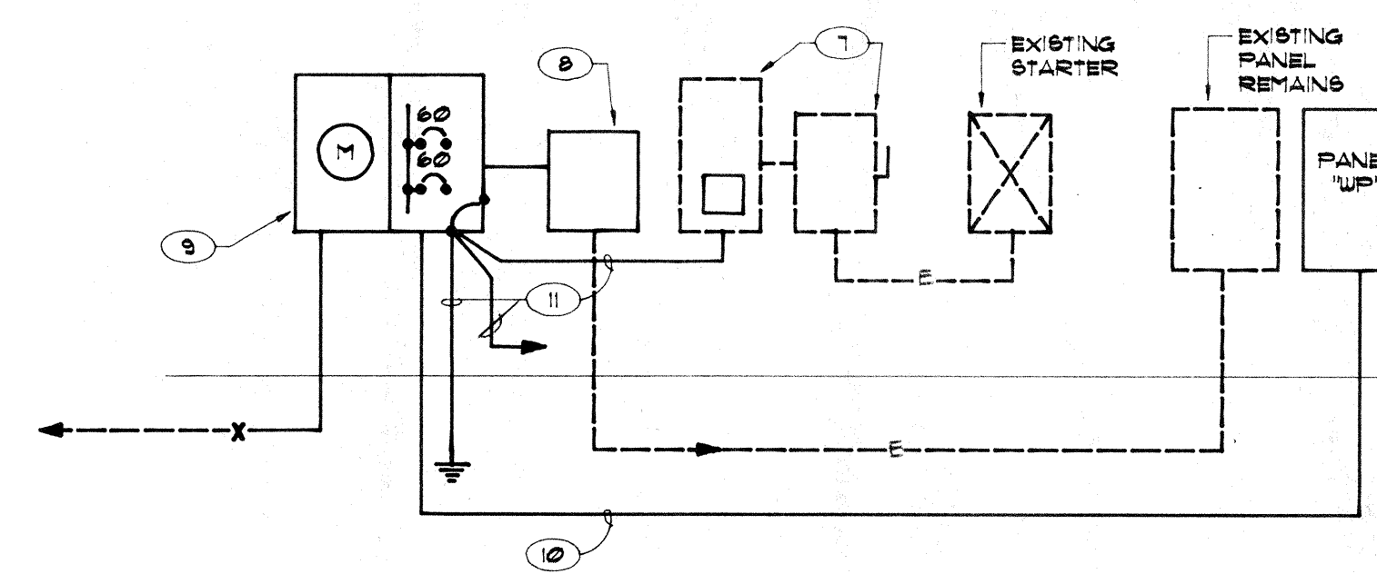
NTB POWER RISER DIAGRAM - NEW WORK
