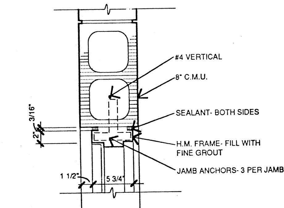
9 Jamb 1 1/2" = 1' - 0"
