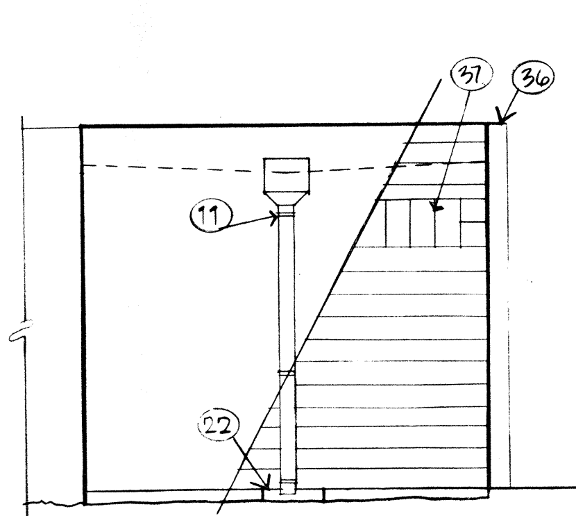
7 East Elevation 1/4" = 1' - 0"
