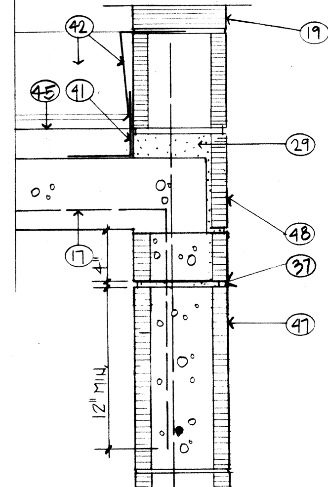
10 Roof Detail 1 1/2" = 1' - 0" (TYPICAL ENTIRE PERIMETER)
