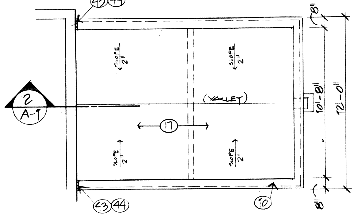
4 Roof Plan 1/4" = 1' - 0"
