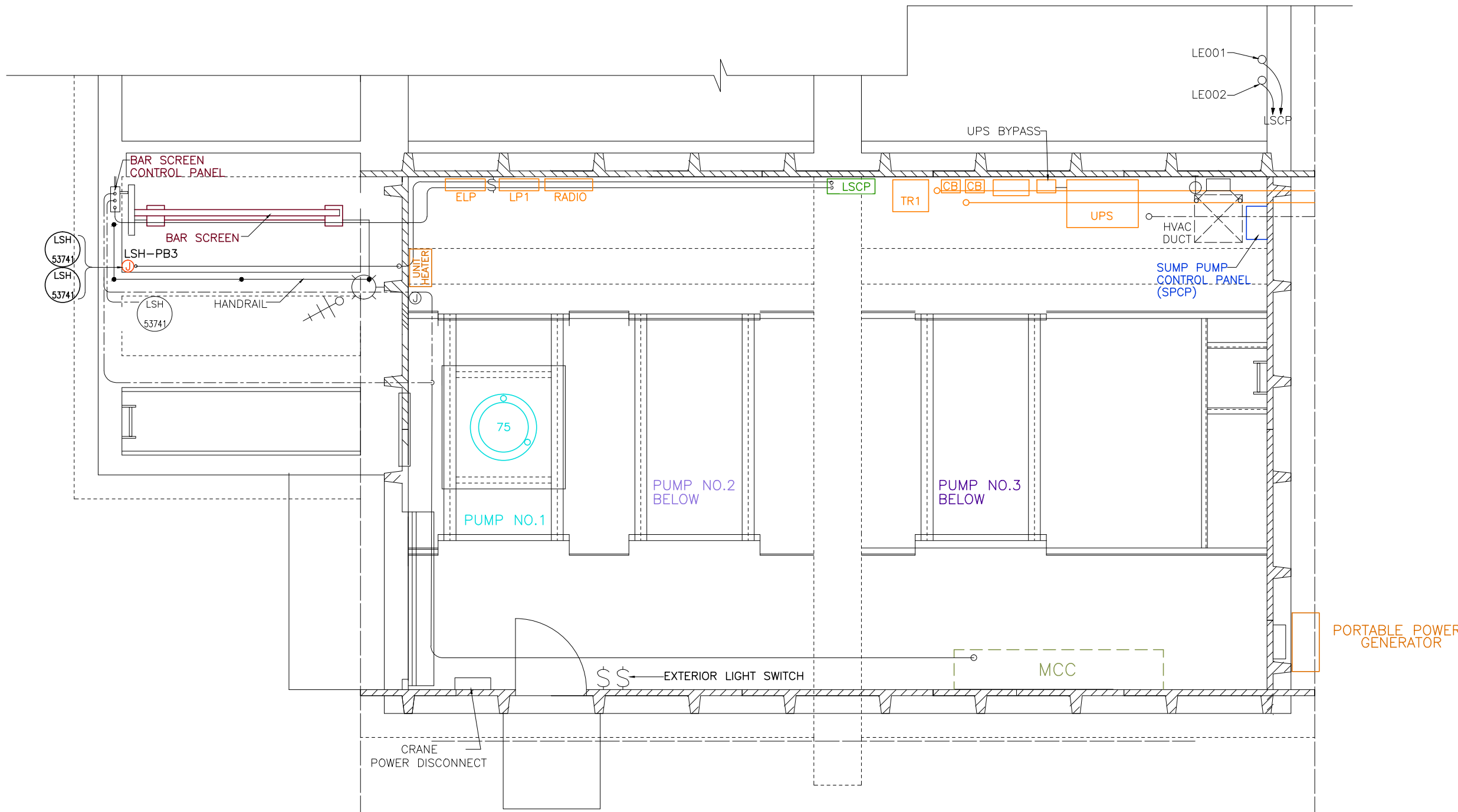
ELECTRICAL SITE PLAN – UPPER LEVEL
