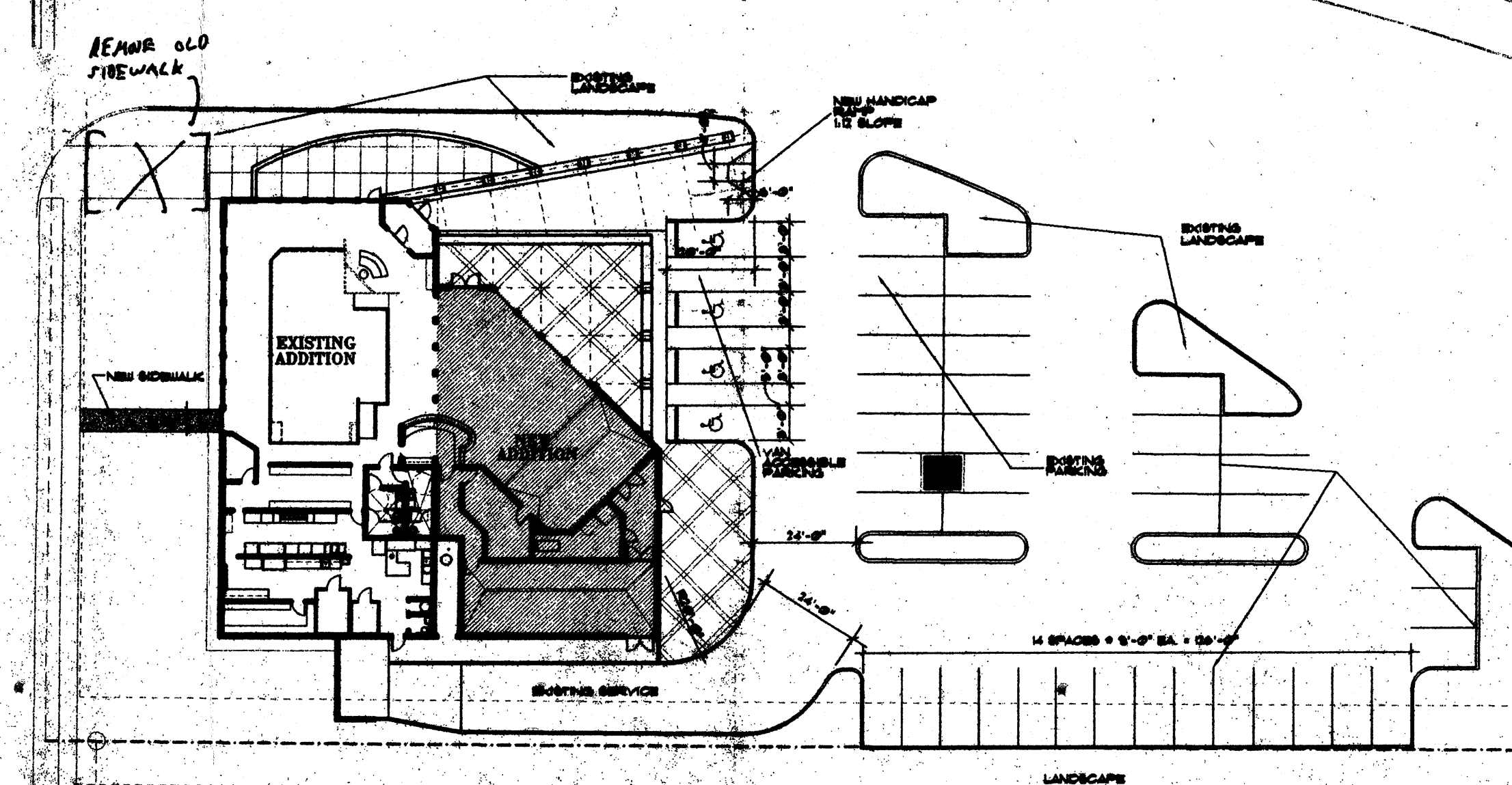
ENLARGED SITE PLAN 1"=30'-0"
