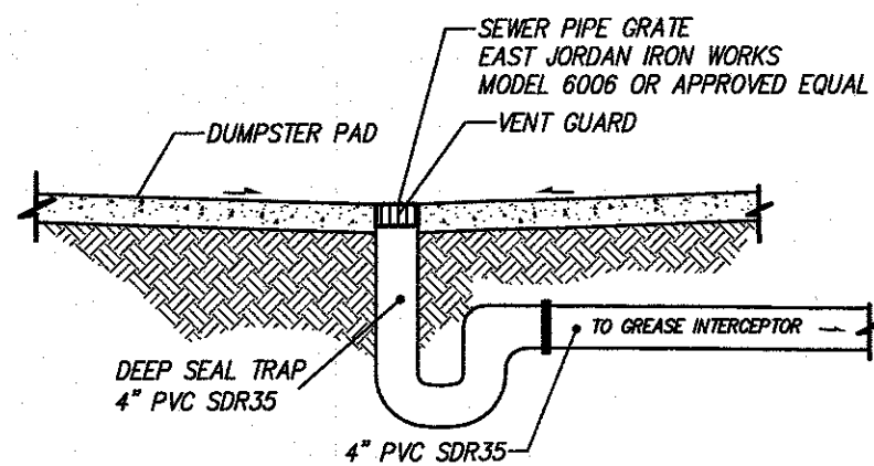
SANITARY SEWER DRAIN FOR REFUSE ENCLOSURE N.T.S.
