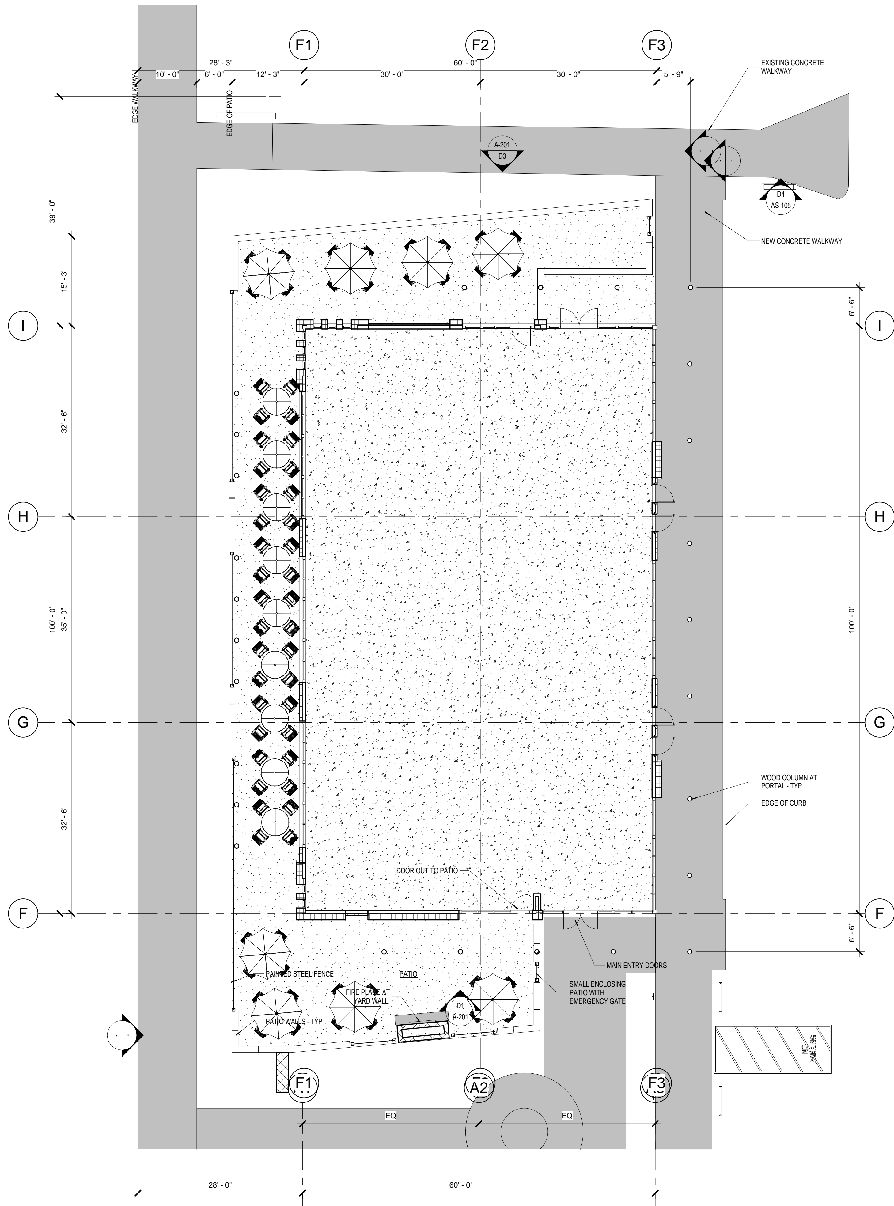
A1 BLDG B - 1ST FLOOR PLAN 1" = 10'-0"
