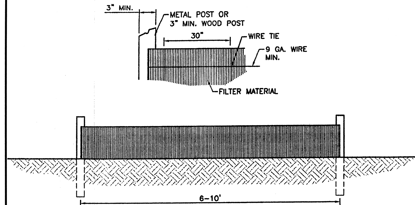
SILTATION FENCE FOR SEDIMENT CONTROL N.T.S.
