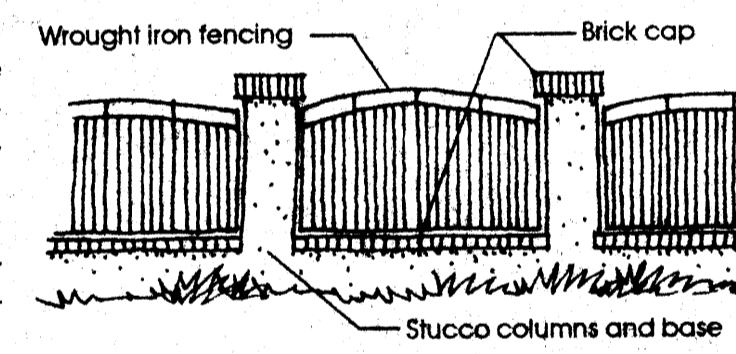
PERIMETER WALL DESIGN
