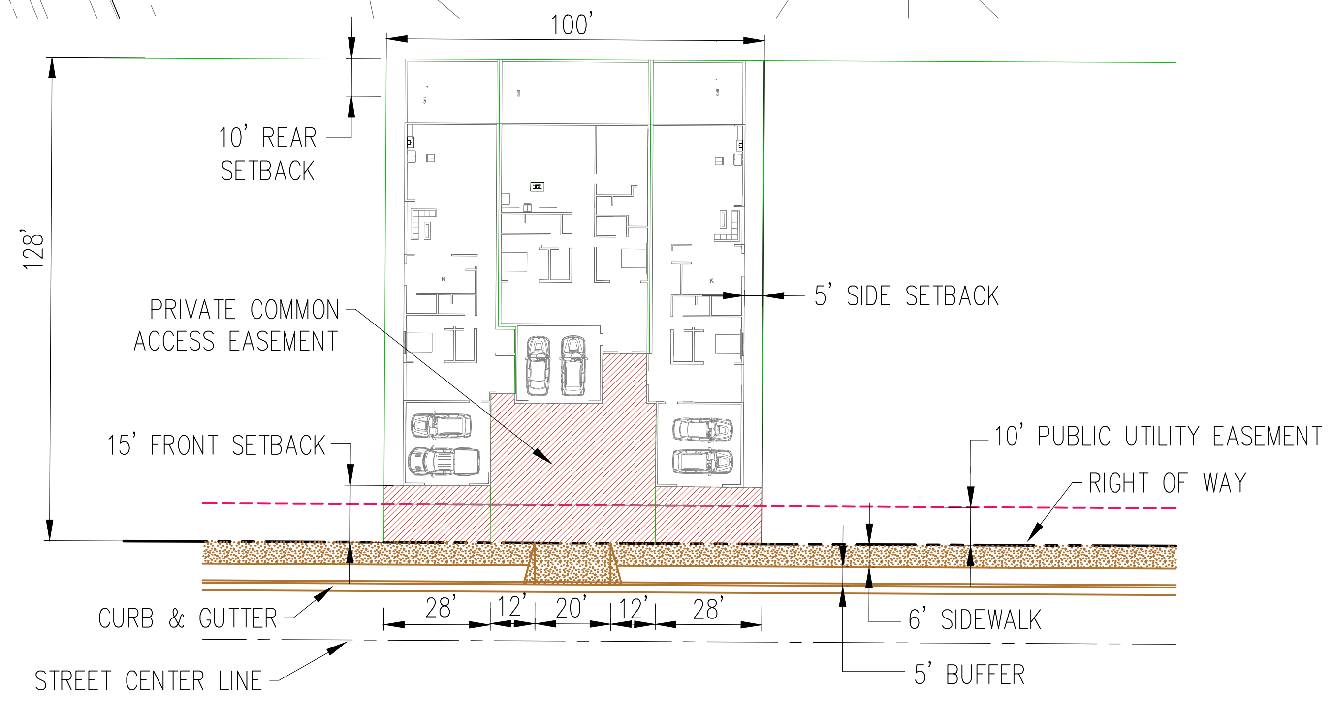
TYPICAL LOT LAYOUT SCALE: NTS
