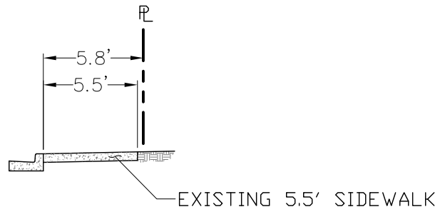
MOUNTAIN ROAD NW TYPICAL SIDEWALK DETAIL
