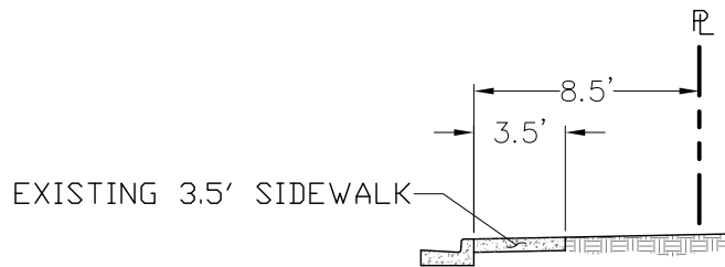
14TH STREET NW TYPICAL SIDEWALK DETAIL
