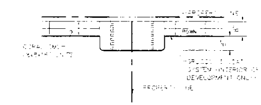
PILASTER PLAN SCALE: 1/4"=1'-0"
