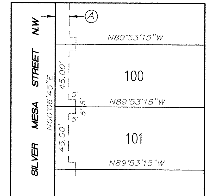
EASEMENT DETAIL AT LOT LINES No Scale
