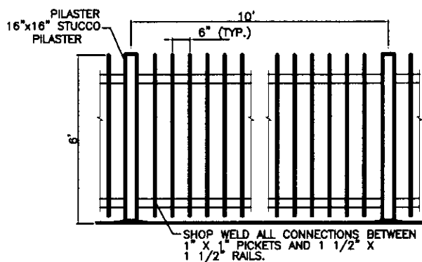
WROUGHT IRON FENCE DETAIL
