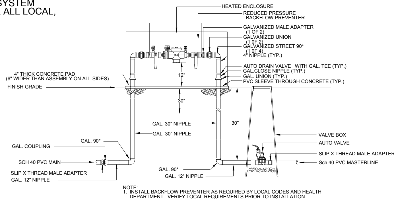
1 RP BACKFLOW/MASTER VALVE DETAIL
