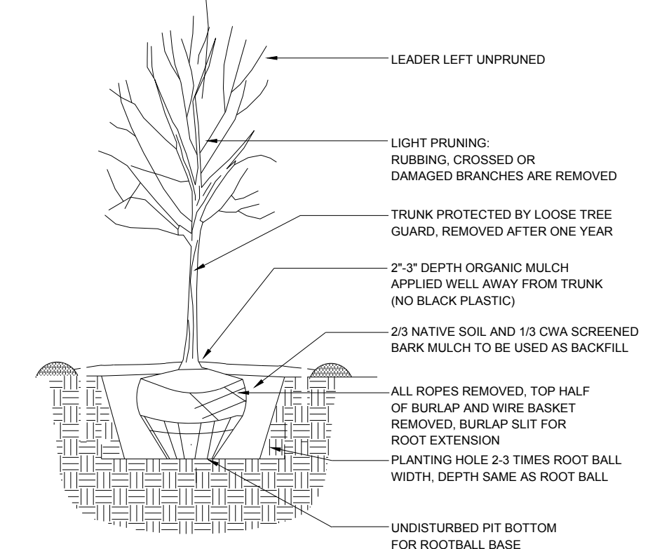
2 TREE PLANTING DETAIL
