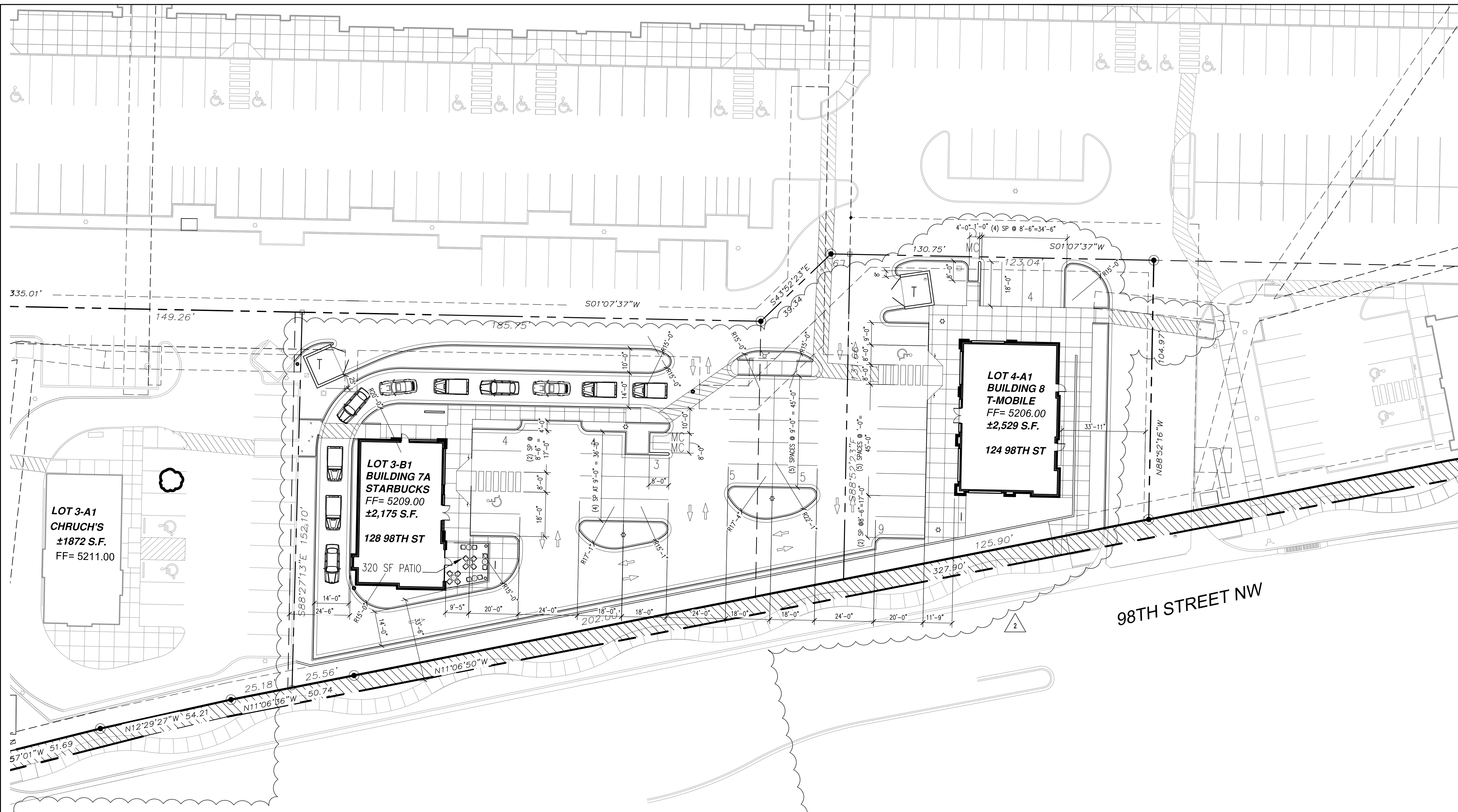
B1 ENLARGED SITE DEVELOPMENT PLAN 1"=20'-0"
