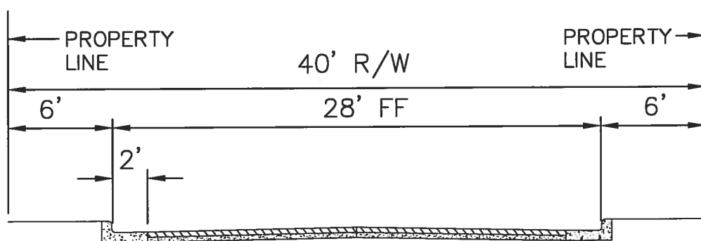
HAMMER HEAD STREETS
