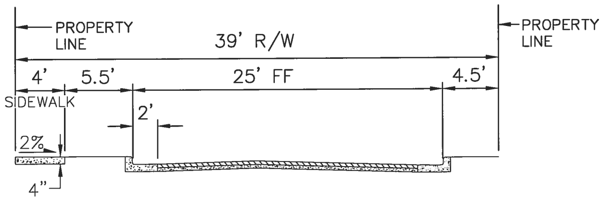
STREETS WITH WAIVED SIDEWALK
