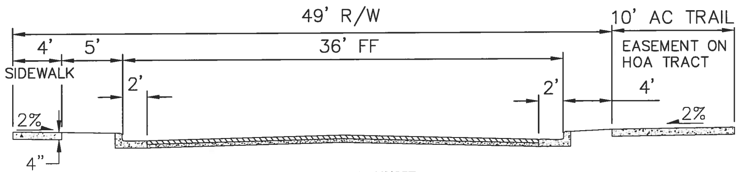
SANDIA SUNSET EAST OF ROCKY TOP DR.
