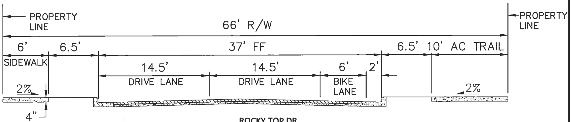
ROCKY TOP DR. AT JUAN TABO DR.
