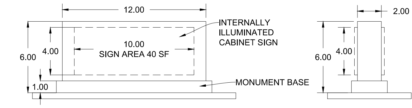
MONUMENT SIGN ELEVATIONS (SIGN TYPE A) N.T.S.
