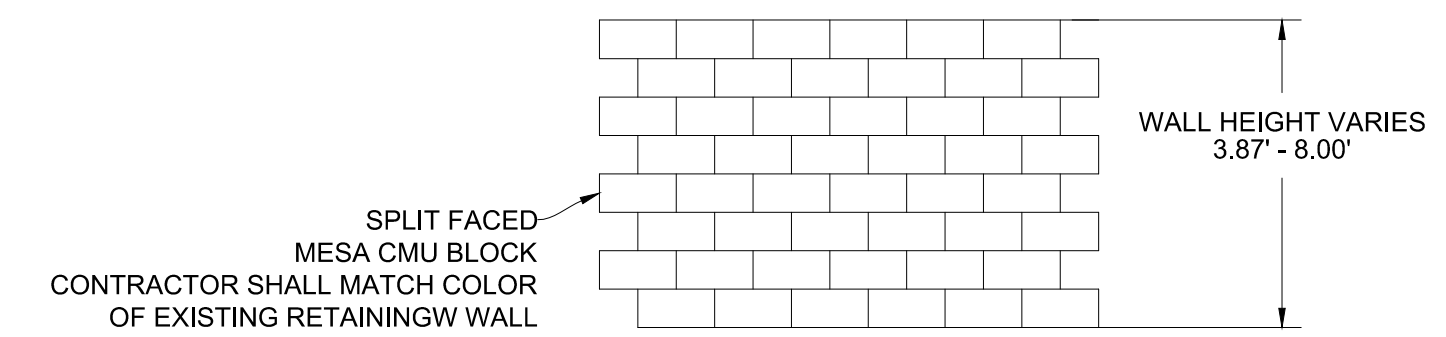
RETAINING WALL ELEV. (TYP SECTION) N.T.S.
