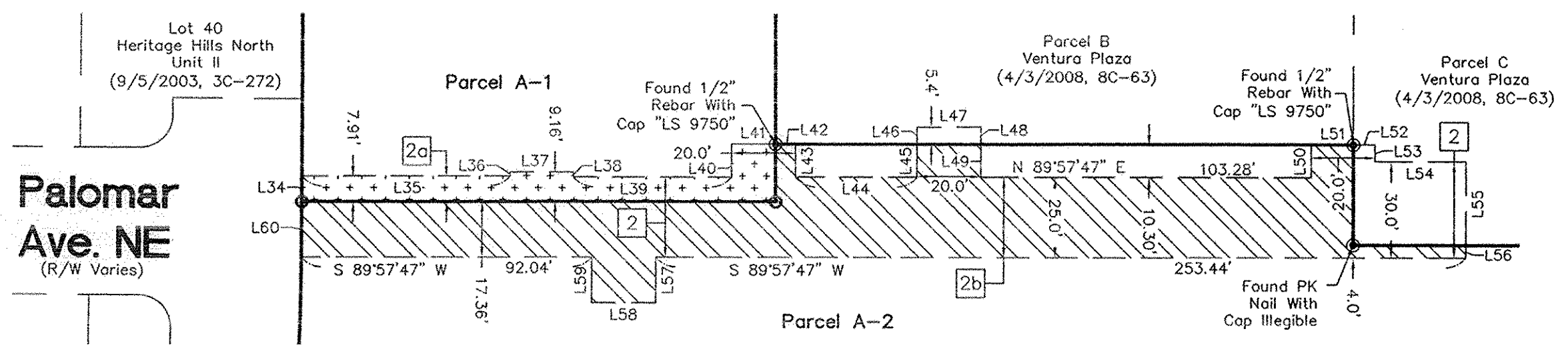
Detail D 1"=40'
