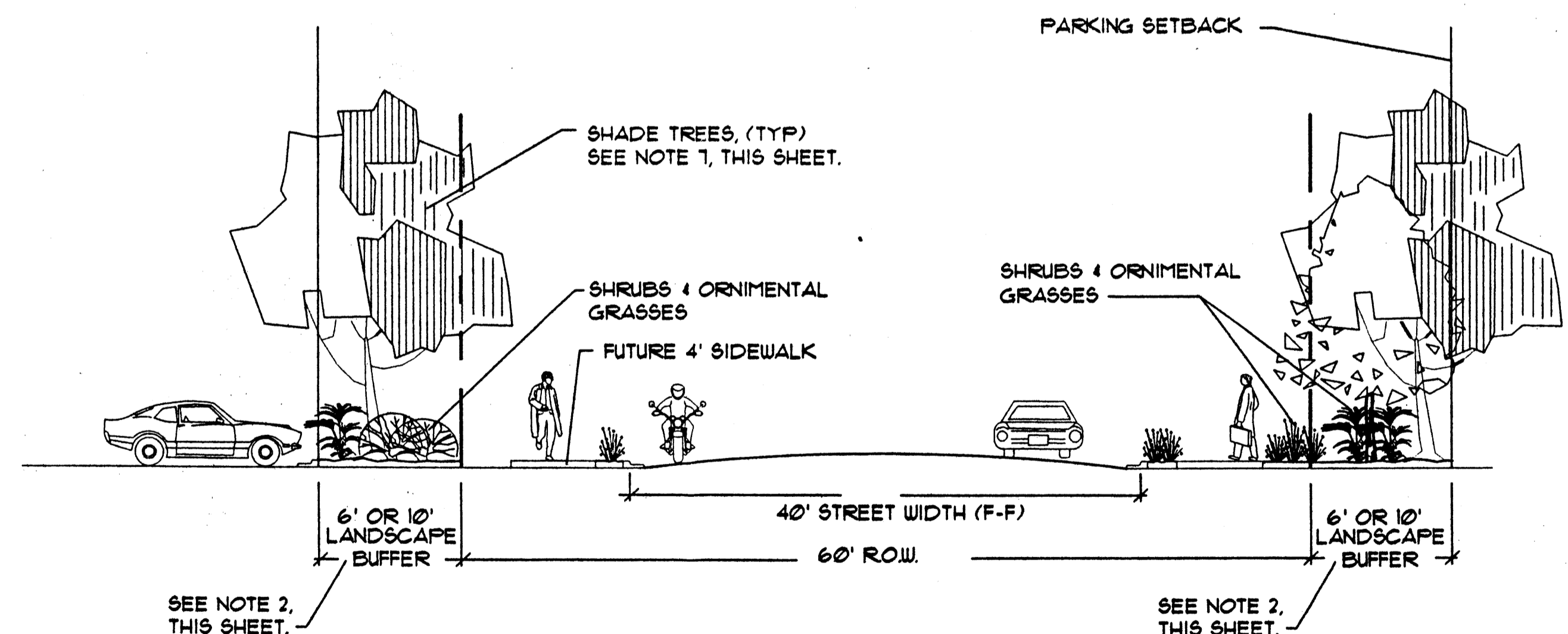
STREETSCAPE TYPICAL SECTION NTS.
