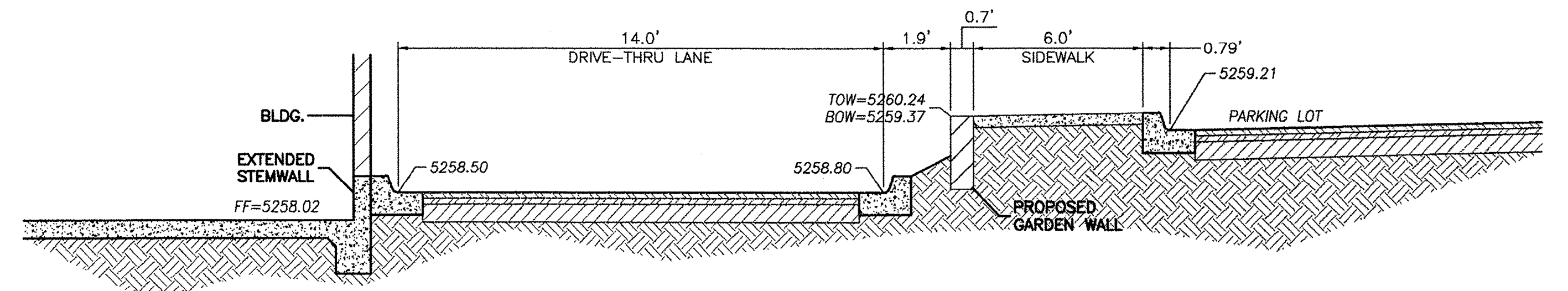
SECTION E-E SC: 1"=3'
