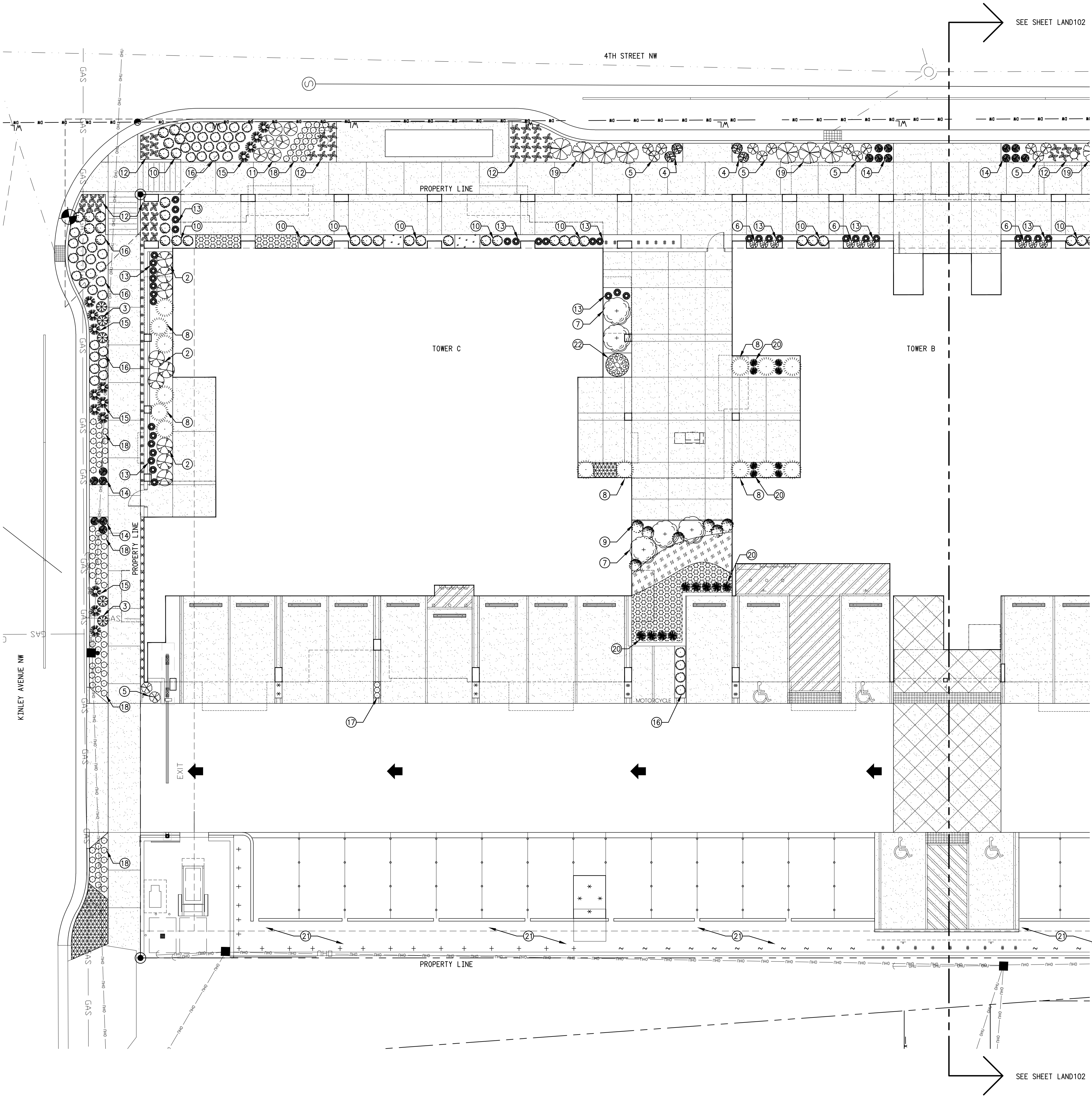
NEW LANDSCAPE PLAN - NORTH - SHRUBS, GRASSES, AND VINES ONLY
