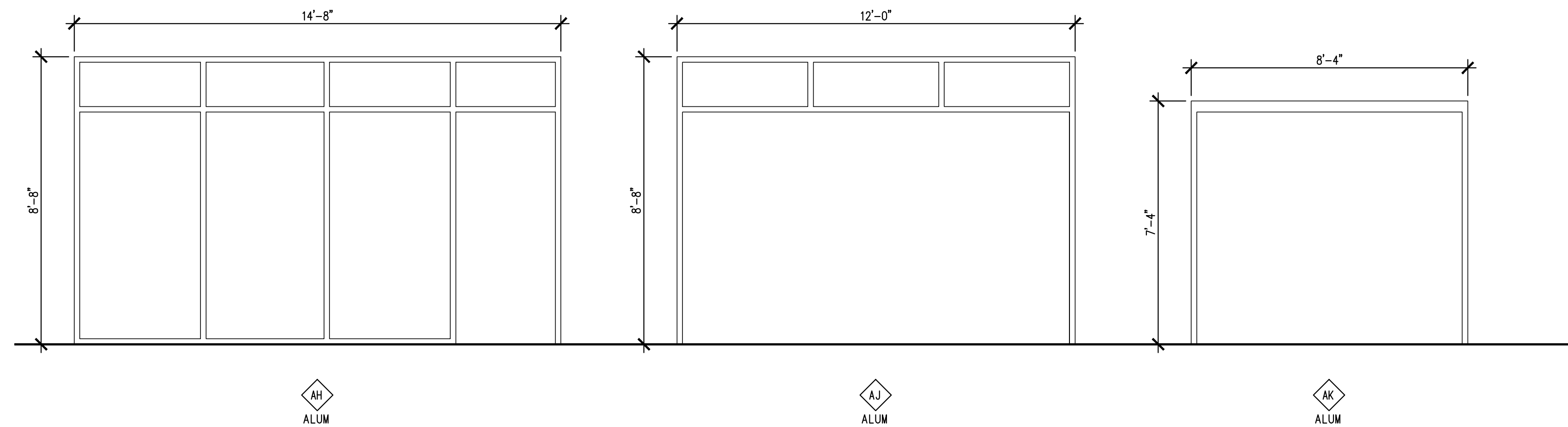
ALUMINUM STOREFRONT FRAME TYPES
