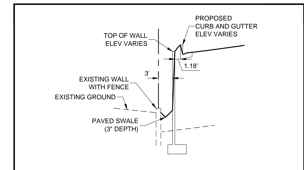
DETAIL 5
