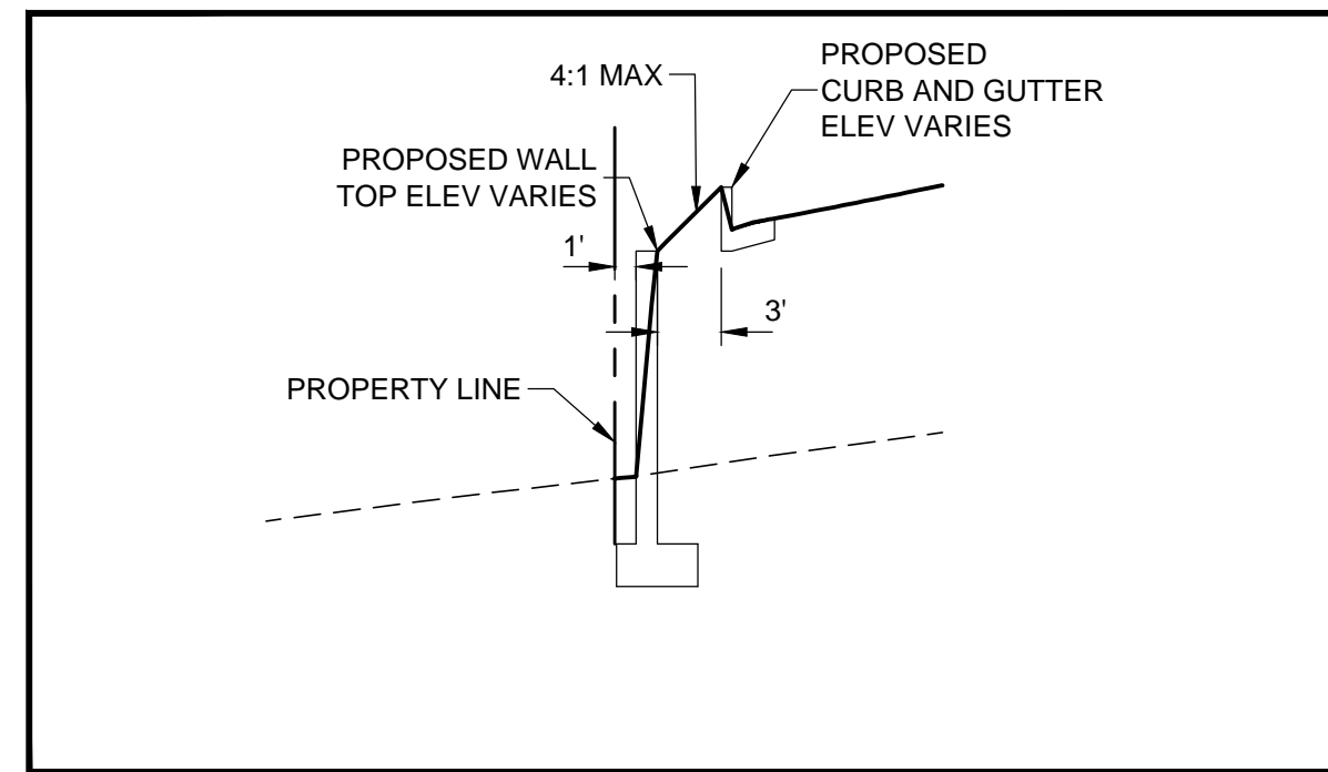
DETAIL 4
