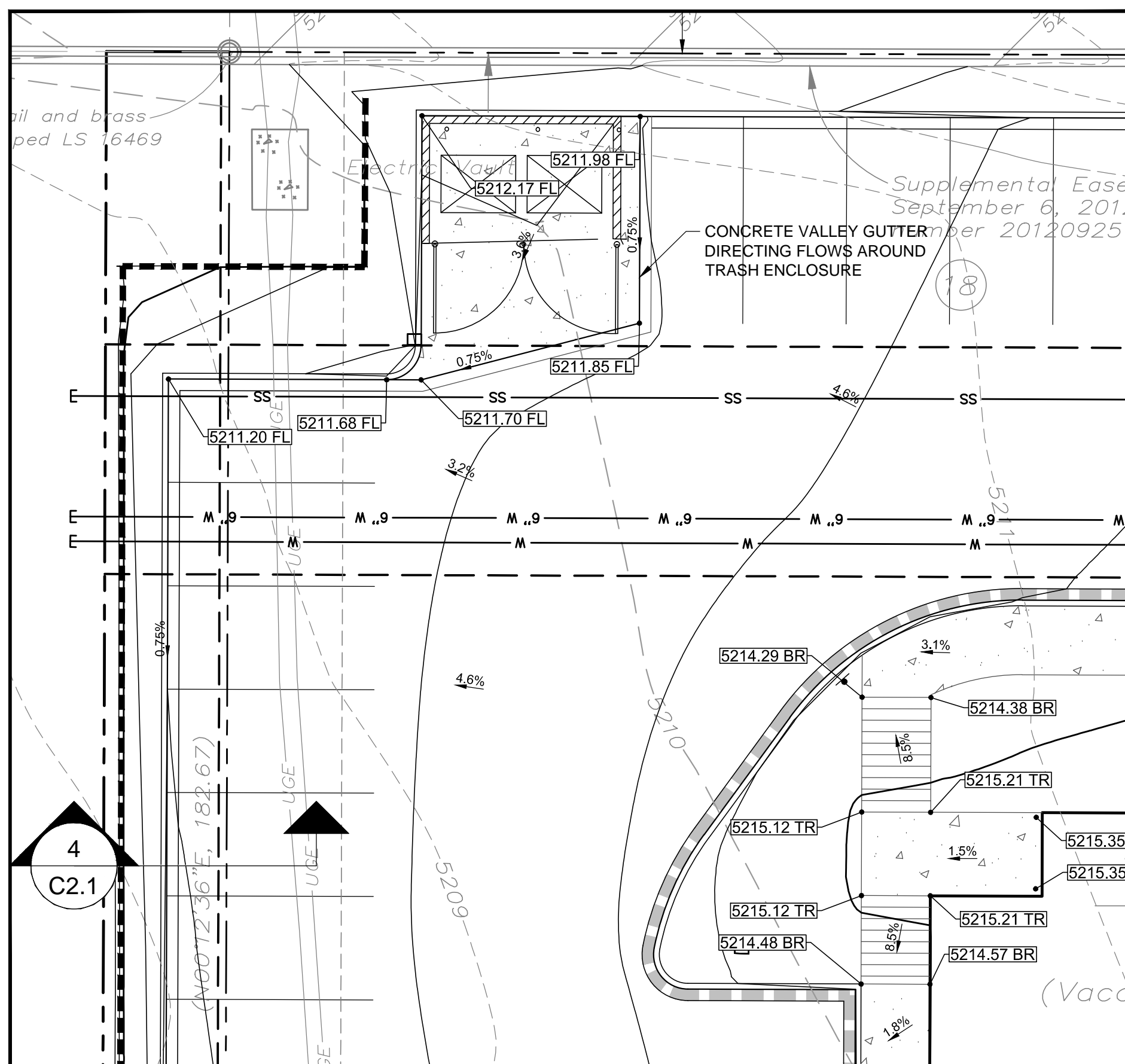
DETAIL 2
