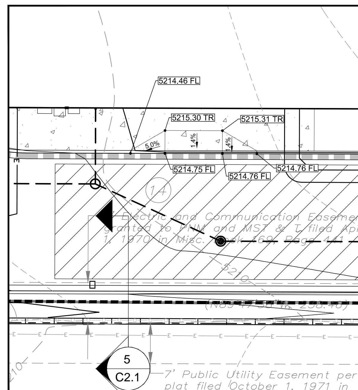
DETAIL 3
