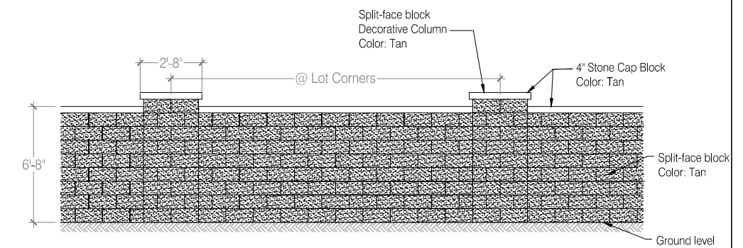
PERIMETER WALL TYPE 'A'
