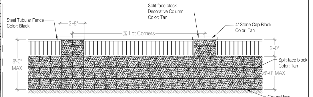
PERIMETER WALL TYPE 'B'
