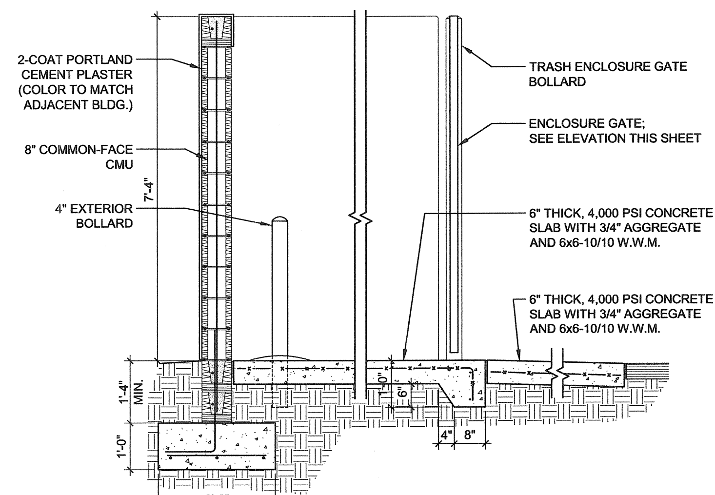
B5 TRASH ENCLOSURE WALL and GATE 1/2" = 1'-0"
