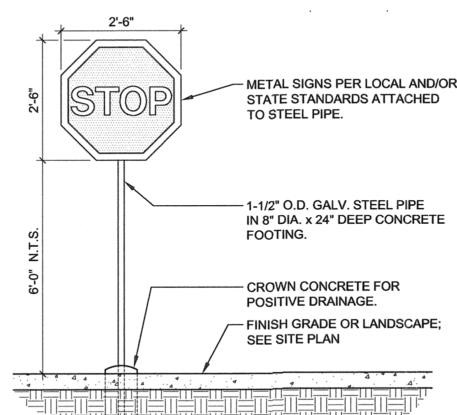
A4 POLE MOUNTED STOP SIGN 1/2" = 1'-0"
