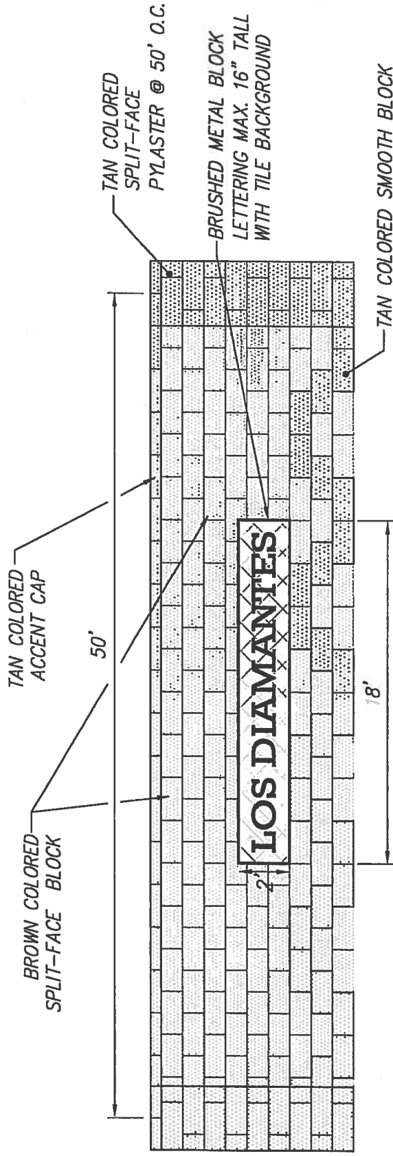
TYPICAL WALL ELEVATION FACING 98TH STREET SW AND BLAKE ROAD SW (SHOWING ENTRY SIGN) NTS
