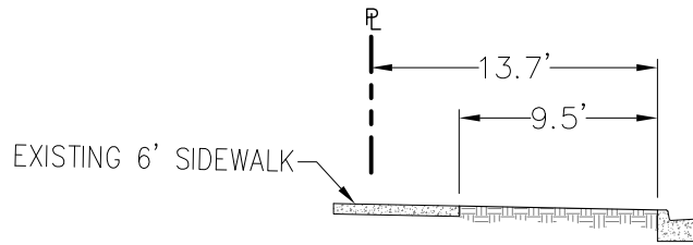
14TH STREET NW TYPICAL SIDEWALK DETAIL
